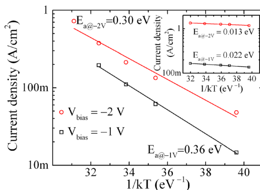
FIG. 3. (Color online) Current density versus 1/kT at 1 V and 2 V reverse bias voltages before annealing. The circular and square symbols are the measured data and the solid lines are the Arrhenius-fit plots. The inset shows the same plot after annealing. The value of the activation energy at each bias voltage is also shown.
