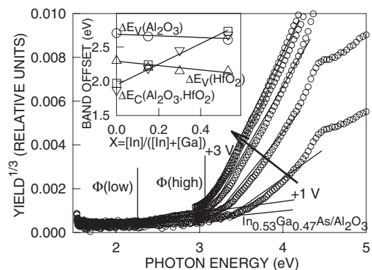
FIG. 4. Cube root of the IPE quantum yield as a function of photon energy as measured in \text{In}_x\text{Ga}_{1-x}\text{As}/\text{Al}_2\text{O}_3(10 \text{ nm})/\text{Au} MIS capacitors under positive bias on the metal electrode increasing from 1 to 3 V in 0.5 V steps. Vertical lines mark two resolved spectral thresholds, \Phi(\text{high}) and \Phi(\text{low}) , corresponding to the direct electron IPE to alumina CB and the IL-assisted transitions, respectively. The inset shows the CB and VB offsets at the interfaces of \text{In}_x\text{Ga}_{1-x}\text{As} with \text{Al}_2\text{O}_3 and \text{HfO}_2 as a function of In content x .
