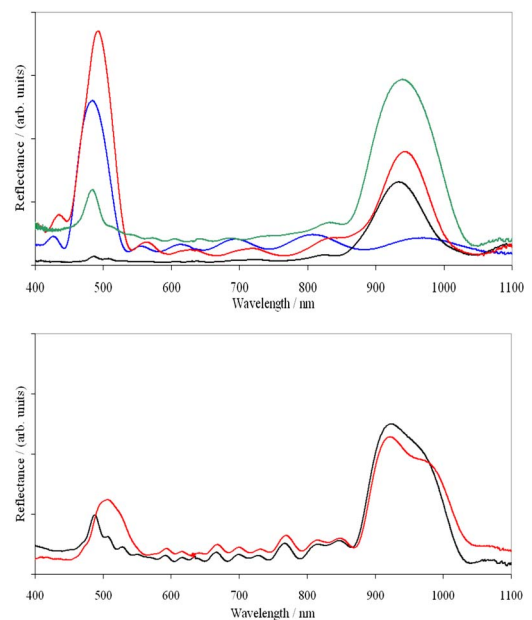
FIG. 3. (a) Reflection spectra of the AB structure taken from the A surface (red) and B surface (black). The reflection spectra of comparable ten layer A only (blue) and ten layer B only (green) crystals are given for comparison. The intensity of the \sim 500 nm peak is clearly enhanced when illuminated from the A surface. (b) Reflection spectra of the BA structure taken from the A surface (red) and B surface (black). Enhancement is not observed and the spectra are complicated by an interface effect.
