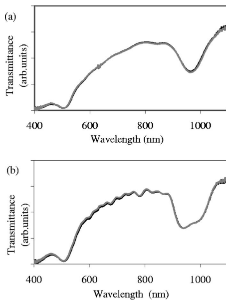
FIG. 1. Transmission spectra of (a) the AB structure and (b) the BA structure taken from both the A and B surfaces. As would be predicted the spectra are not dependent on the direction of illumination.
