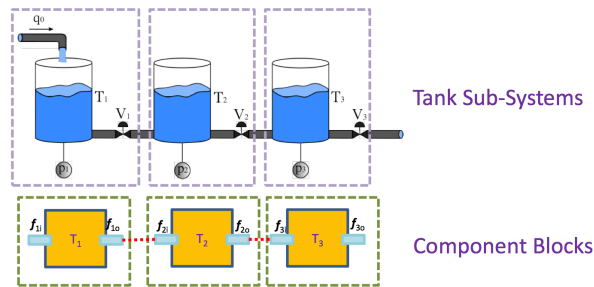
Fig. 3. Diagram of the three-tank system.
