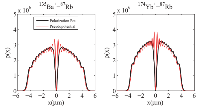
FIG. 3. (Color online) The single-particle densities of a TG gas of 20 particles in the presence of a central ion for ^{135}\text{Ba}^+ \text{-} ^{87}\text{Rb} and ^{174}\text{Yb}^+ \text{-} ^{87}\text{Rb} systems with a typical trapping frequency, \omega = 70\text{Hz} (thick black line). The short range phases in each case are chosen to be \phi_e = \frac{\pi}{4} and \phi_o = -\frac{\pi}{4} . The thin red line in the plots represents the result of a pseudopotential approximation for the ion, using a large value for the scattering length.
