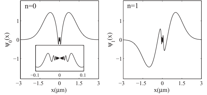
FIG. 2. The first two trap states of a harmonic trap with a centrally embedded ion for a ^{135}\text{Ba}^+ \text{-} ^{87}\text{Rb} system for axial trapping frequency, \omega = 70\text{Hz} . The inset for the n = 0 state shows a zoom in of the region around zero where the wave function is rapidly oscillating. The short-range phases are chosen to be \phi_e = \frac{\pi}{4} and \phi_o = -\frac{\pi}{4} .
