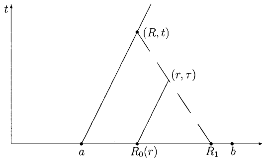
FIG. 2. Solid lines \bar{\Gamma}_a, \bar{\Gamma}_{R_0(r)} are outgoing null curves. The dashed line is \Gamma_{R_1} , an ingoing null curve.
