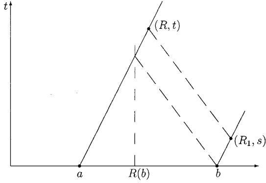
FIG. 1. Solid lines \bar{\Gamma}_a, \bar{\Gamma}_b are outgoing null curves. Dashed lines are ingoing null curves \Gamma_b, \Gamma_{(R_1, s)} .
