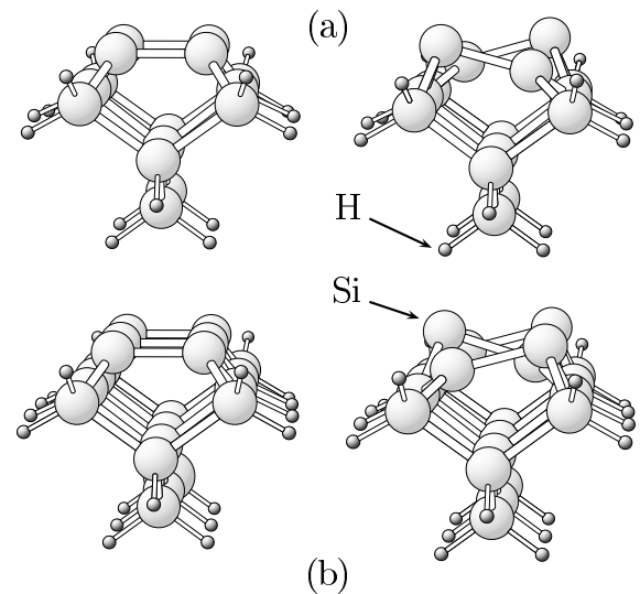
FIG. 2. \text{Si}_{15}\text{H}_{16} (a) and \text{Si}_{21}\text{H}_{20} (b) cluster models of the Si(100) surface. Both the symmetric (left) and buckled (right) reconstructions are shown.
