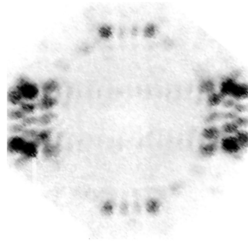
FIG. 4. Far field of the laser at 1.6 times lasing threshold, showing both the polarization and the multimode instabilities.
