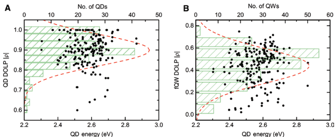
Figure 4: The 180 a -plane InGaN/GaN (A) QD and (B) underlying QW DOLP variation with emission energy. The statistical distributions have been fitted with Gaussian profiles. The means and standard deviations of the Gaussian distributions are (A) 0.90 \pm 0.08 and (B) 0.46 \pm 0.14 , respectively.
