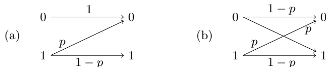
Fig. 1. A Z-channel (a) and a standard Binary Symmetric Channel (b).
