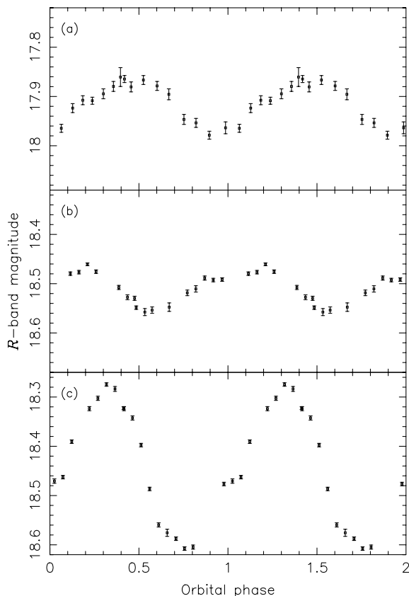
Figure 2. R -band light curves, folded on the pulse timing ephemeris (Kaaret et al. 2006), and plotted twice for clarity. (a) ATT light curve from 2006 September 21, (b) LBT light curve from 2007 June 13, (c) LBT light curve from 2007 June 24.
