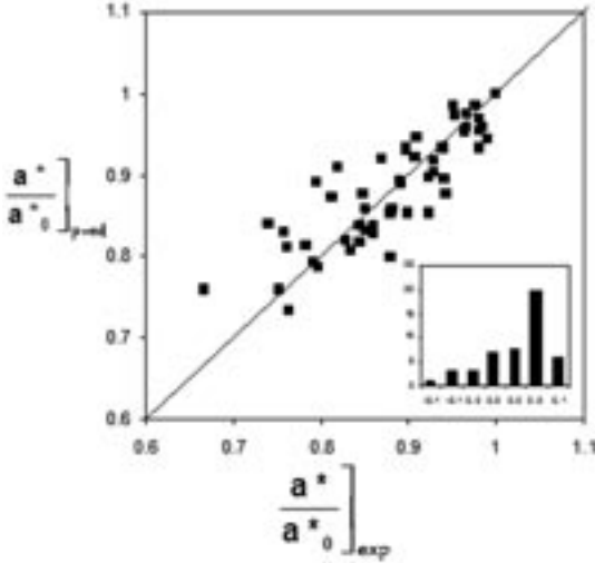
Fig. 4 - Relationship between experimental and predicted values of the colour ( a^*/a_o^* ) measured during storage of shredded carrots in air flux system in a range of temperature 0°-20°C. Enclosed figure: Frequency distribution of the residual.
