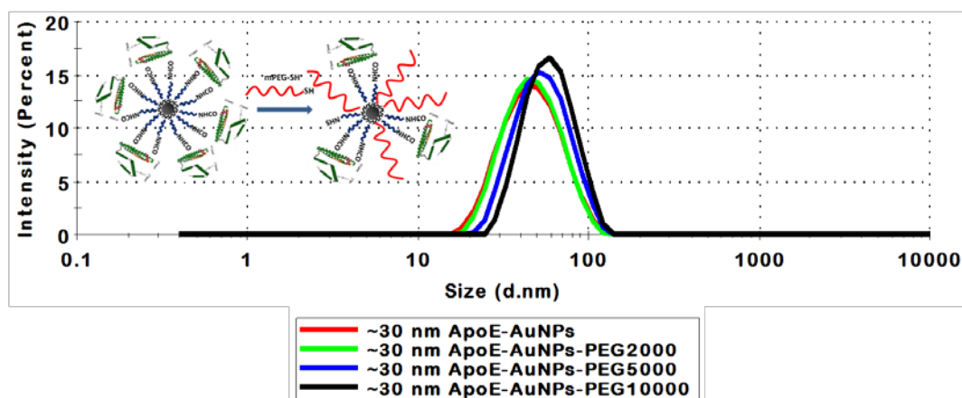
Figure 7. Size distribution by intensity obtained from DLS on 30 nm Au NPs-PEG-NHCO-ApoE (ApoE-AuNPs) before, and after PEGylation with mPEG-SH ( M_w \sim 2100 , 5400 and 10000 g\ mol^{-1} ) insert show the overall process Scheme 2).
