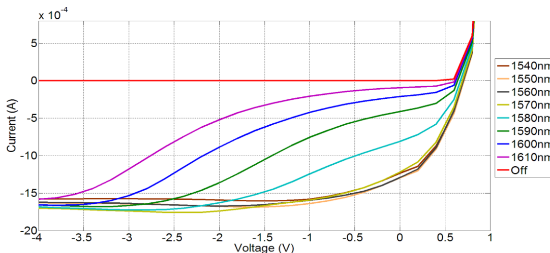
Fig. 5.24: EAM absorption for an off-chip tuneable laser source.
