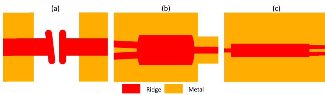
Fig. 3.1: Schematic of cells containing a (a) T bar slot (b) 2x1 star coupler (c) 1x2 MMI.
