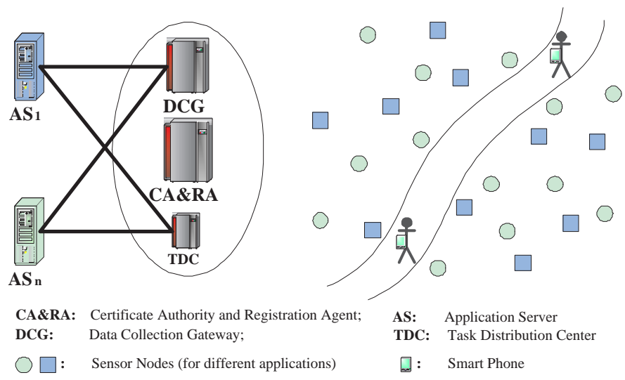
Fig. 2. The Architecture of SOI
