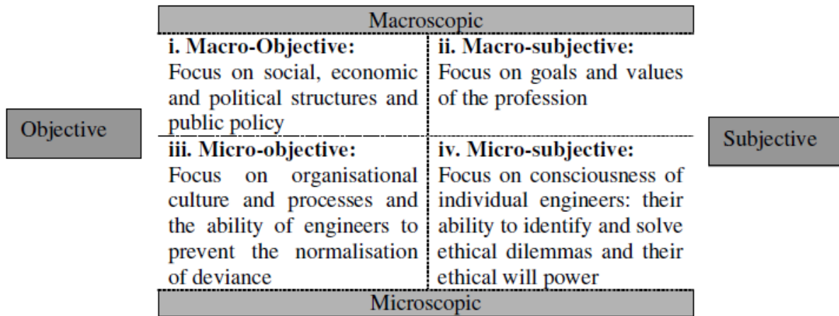
Fig. 1. Conlon's four quadrant model for engineering ethics (Conlon, 2010)
