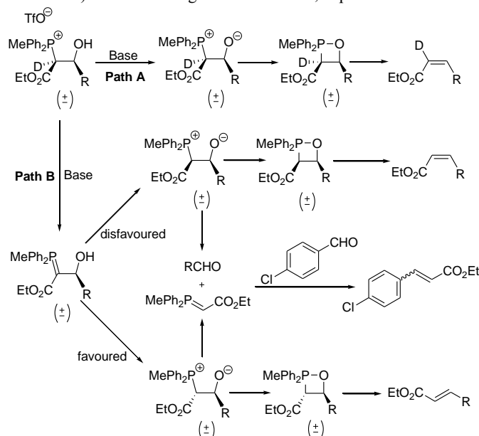
5 Scheme 19. Experiments on \alpha -deuterated erythro - \beta -HPSs. R = Ph, \text{CH}_2\text{CH}_2\text{Ph} , c\text{-C}_6\text{H}_{11} , or \text{CMe}_2\text{CH}_2\text{Ph} . 60
