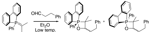
Scheme 21. Wittig reaction of iso-propyldenediphenyldibenzophospholane with 3-phenylpropanal to give OPA pseudorotamers that are distinguishable by NMR.
