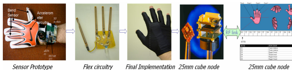
Fig. 5. 25mm Tyndall wireless sensor enabled glove prototype & GUI development cycle.
