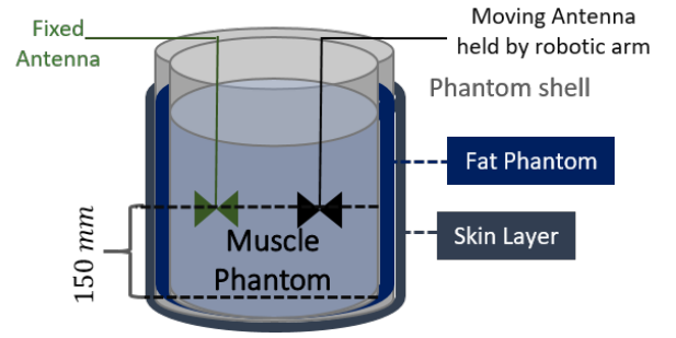
Fig. 3. Illustration of experimental setup showing tissue layers.
