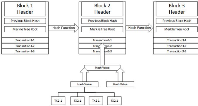
Figure 1. Blockchain Structure
