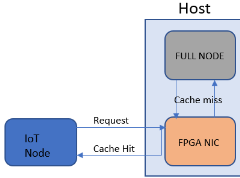
Figure 2. FPGA NIC in IoT environment
