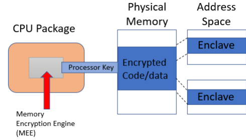
Figure 3. SGX Enclave
