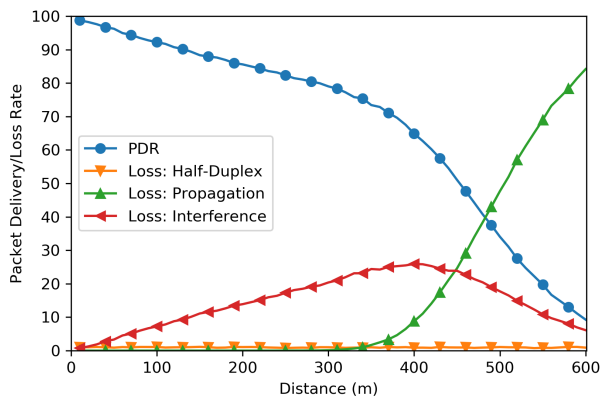
Fig. 5: PDR & Causation of Packet Loss (Highway Fast)
