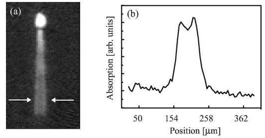
FIG. 2. (a) Atom laser beam extracted from a compressed Bose-Einstein condensate. The double peak structure of the beam is clearly visible. The height of the image is 780 \mu\text{m} . (b) Cut through the atomic density distribution at the position indicated by the arrows.
