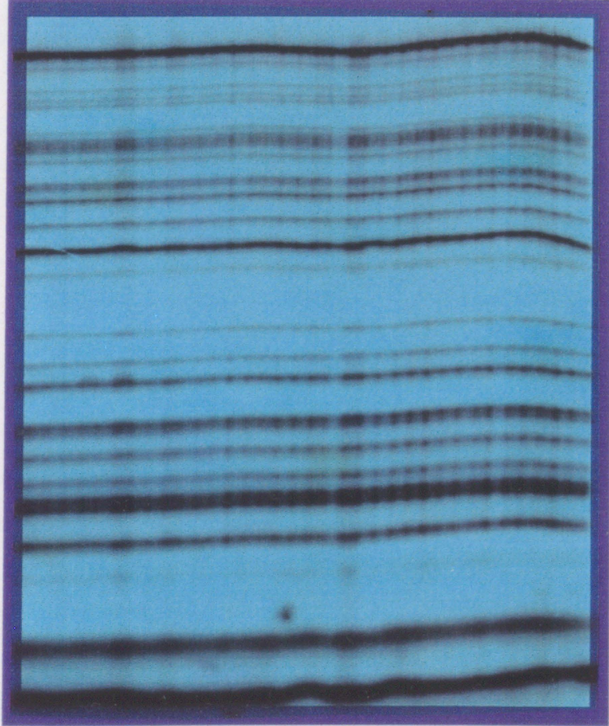
Figure 2.10. Autoradiograph showing the GMPD-scan analysis of matched normal and tumour DNA from 15 sporadic colon cancer patients. Exon 1 of the K-ras 2 gene was amplified from 20 matched normal and tumour DNA samples (not all shown), in a reaction containing unlabelled primer R and \gamma^{32} labelled primer F. Following amplification, GMPD analysis was performed on all samples and digestion products were separated in a 10% denaturing polyacrylamide gel. Normal (N) and tumour (T) DNA samples were loaded as indicated.
