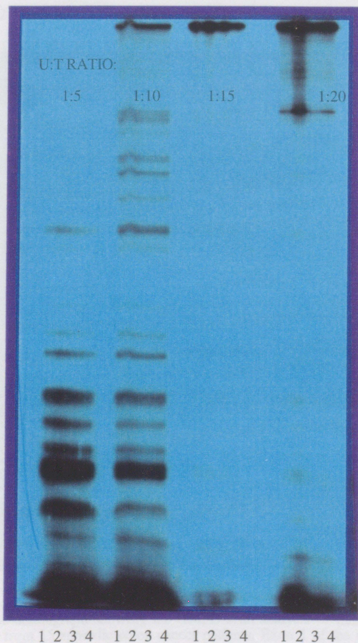
Figure 2.9. Optimisation of the U:T ratio for GMPD-scan analysis. Exon 1 of the k-ras 2 gene was amplified from 4 DNA samples in a PCR reaction containing \gamma^{32}\text{P} labelled primer F and unlabelled primer R. The reaction was performed with U:T ratios of 1:5, 1:10, 1:15, 1:20 as indicated. Following amplification, GMPD analysis was performed on each sample, digestion products were separated in a 10% denaturing polyacrylamide gel and visualised by autoradiography.
