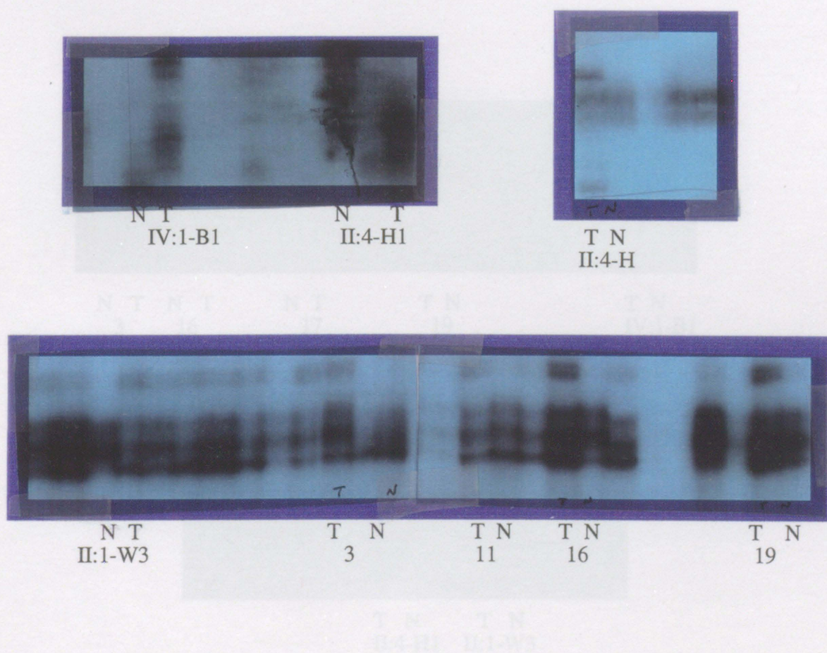
Figure 3.4. Analysis of DNA instability at the 26bp polyA tract at the BAT 26 locus. The Bat 26 locus was amplified from normal (N) and tumour (T) DNA in a PCR reaction containing the BAT 26 forward and reverse primers. \alpha - ^{32}\text{P} dCTP was included in the reaction to label the PCR products. Products were separated in a 6% denaturing polyacrylamide gel and visualised by autoradiography. Matched normal and tumour DNA from 38 samples were analysed (not all shown). Instabilities were observed in HNPCC samples: IV:1-B1, II:4-H1, II:4-H and II:1-W3 and in sporadic colon cancer samples 3, 11, 16 and 19. Only matched samples displaying differences are numbered.
