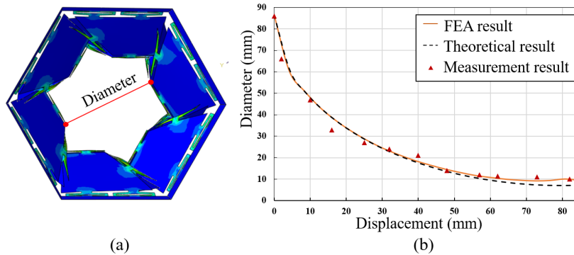
Fig. 9. (a) Top view of the simulation model, the diameter is the distance between the central point P of two opposite folding units. (b) The diameter-displacement curves during folding.
