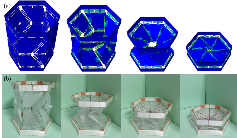
Fig. 7. (a) The inward folding process of the RC-kiri simulation model. (b) The inward folding process of the 3D printed model. (video)
