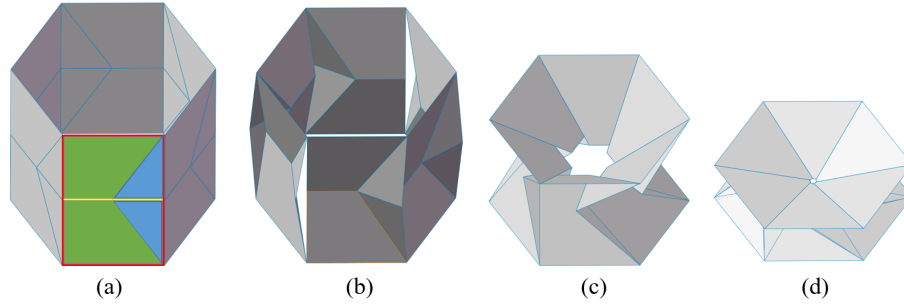
Fig. 2. The folding process of the RC-kiri structure [6]
