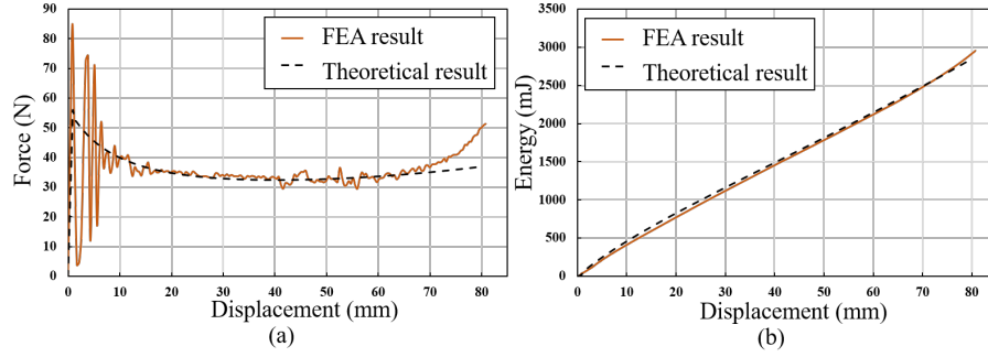
Fig. 6. (a) Force-displacement curves of both theoretical result and simulation result of inward folding RC-kiri. (b) Energy-displacement curves of inward folding RC-kiri.
