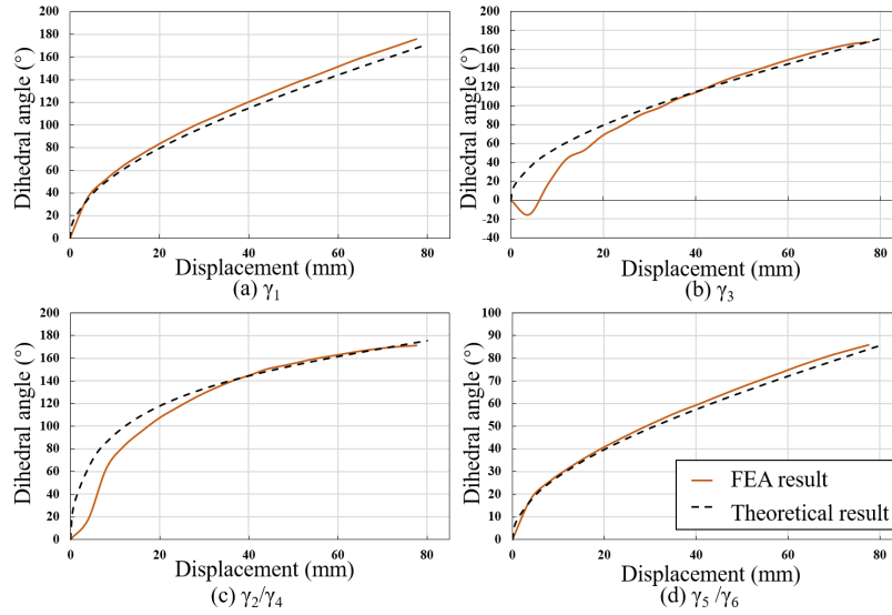
Fig. 8. The dihedral angles between each facet.
