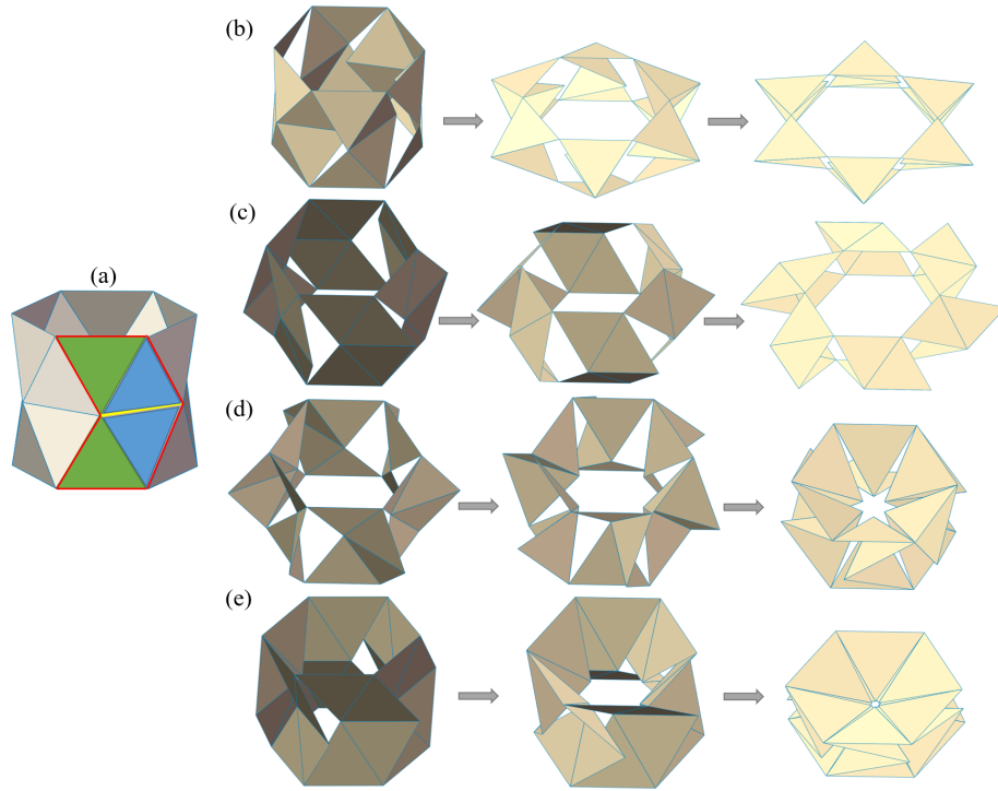
Fig. 1. (a) Tubular Yoshimura structure. (b-e) The folding process of four configurations of tubular Yoshimura kirigami structure.
