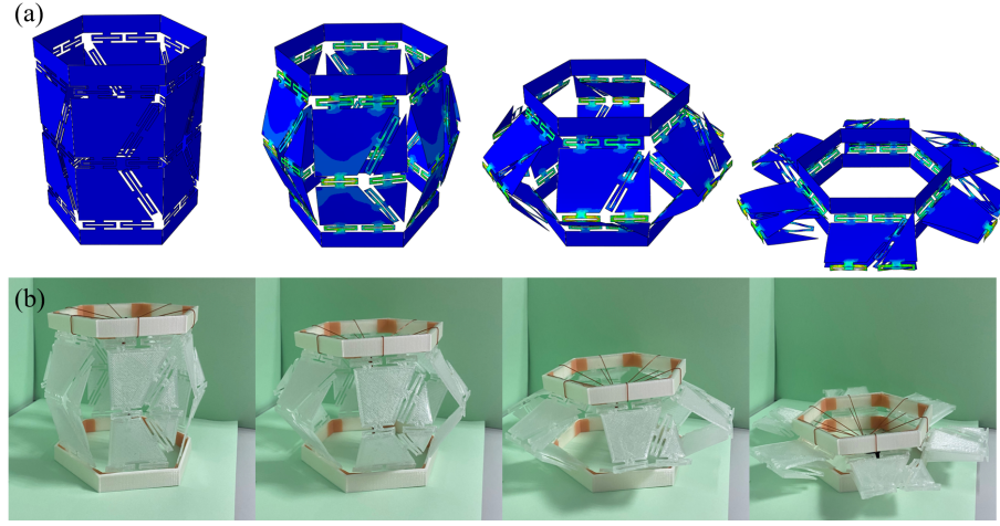
Fig. 10. (a) The outward folding process of the RC-kiri simulation model. (b) The outward folding process of the 3D printed model.
