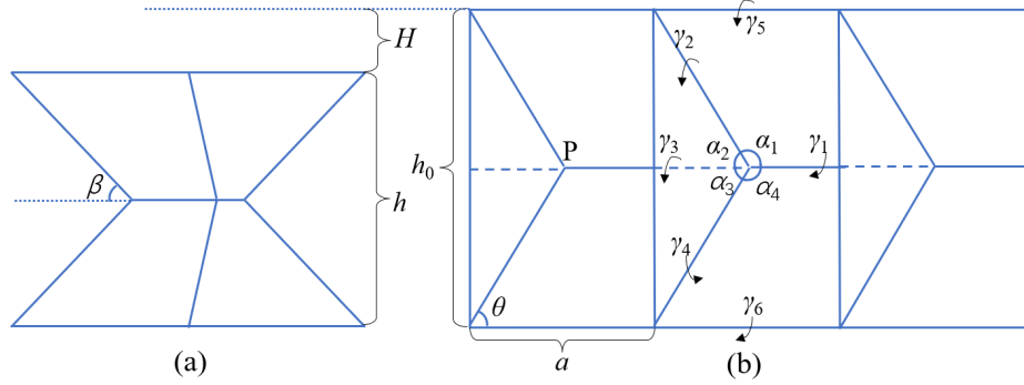
Fig. 4. (a) Front view of the RC-kiri structure. (b) RC-ori crease pattern.
