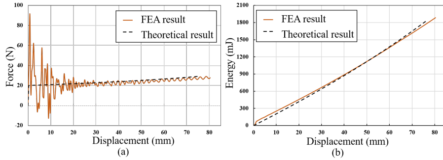
Fig. 11. (a) Force-displacement curves of both theoretical result and simulation result of outward folding RC-kiri. (b) Energy-displacement curves of outward folding RC-kiri.
