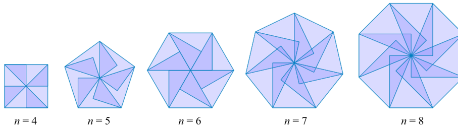
Fig. 3. The top view of fully folded RC-kiri when n = 4, 5, 6, 7, 8 . Darker areas represent more overlapping layers.
