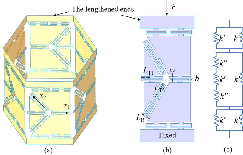
Fig. 5. (a) The tubular RC-kiri model with outside LET joints. (b) Marks for folding unit related parameters. (c) Equivalent spring model of a folding unit.
