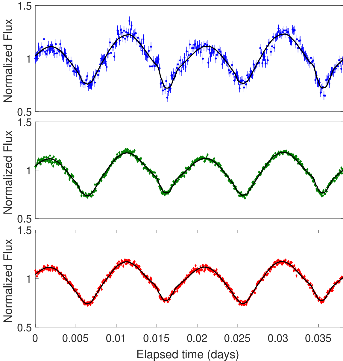
Figure 5. Three-color ULTRACAM light curve from 2023 March 20, overlaid with the best-fit toy LCURVE model (solid black lines). The model includes contributions from an accretion disk and a hot spot where the accretion stream intersects the outer disk, which were needed to achieve an acceptable fit to the light curve. The best-fit model gives a near-edge-on inclination ( 88.6^\circ ), though we chose not to include this model as part of our joint fit due to the large number of model-dependent free parameters involved, as compared to our more simple and robust approach.
