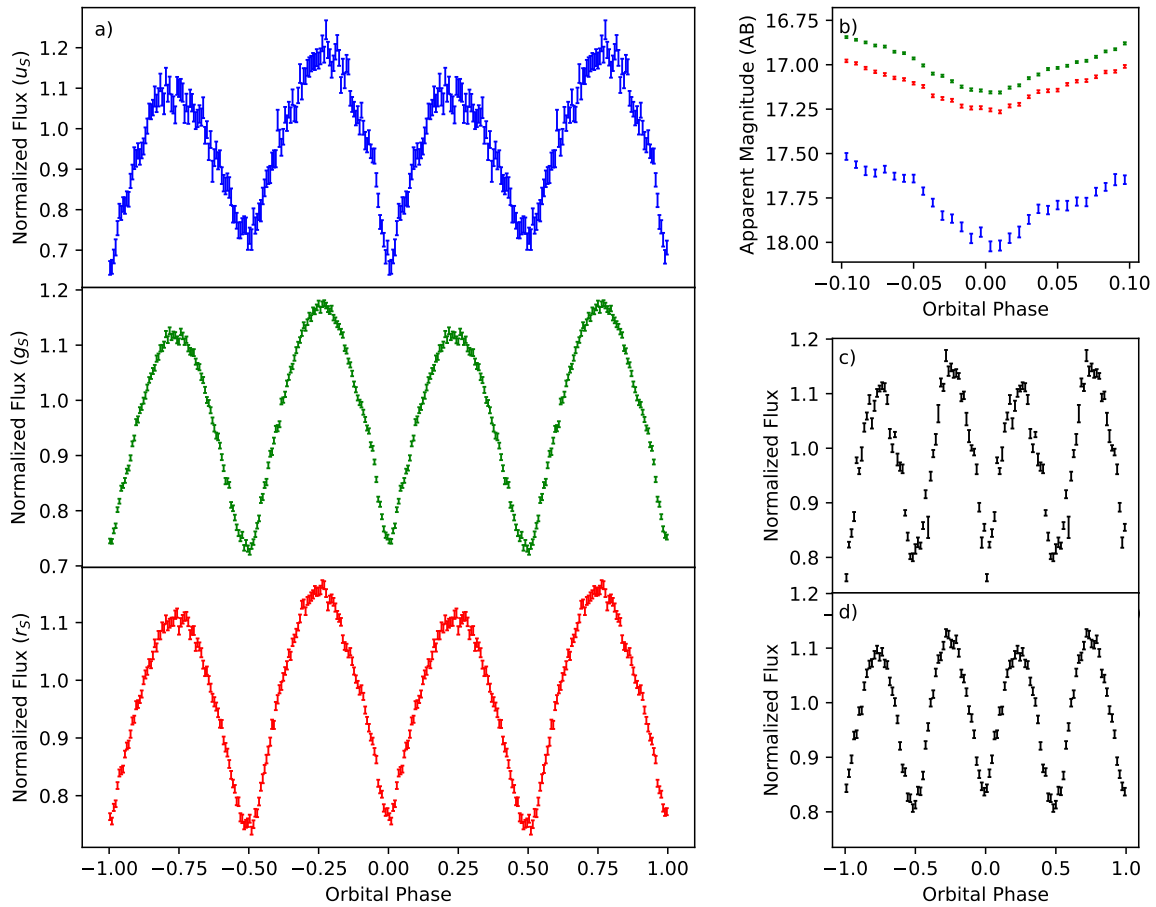
Figure 1. Light curve of ATLAS J1138-5139. (a) The binned u_s g_s r_s ULTRACAM light curve of ATLAS J1138-5139, phase-folded on the 27.68 minutes orbital period. The light curve exhibits sinusoidal variations, with maxima at phases 0.25 and 0.75, due to an ellipsoidally deformed secondary star. At phase 0.75, a heated accretion feature contributes additional flux, resulting in the appearance of unequal maxima. (b) The asymmetric primary eclipse in the u_{gr} ULTRACAM light curve, indicating the presence of a luminous hot spot on the outer edge of an accretion disk surrounding the primary star. (c) The binned and phase-folded light curve of the object from ATLAS. We were able to discover the object because of its periodic behavior. (d) The binned and phase-folded TESS light curve.
