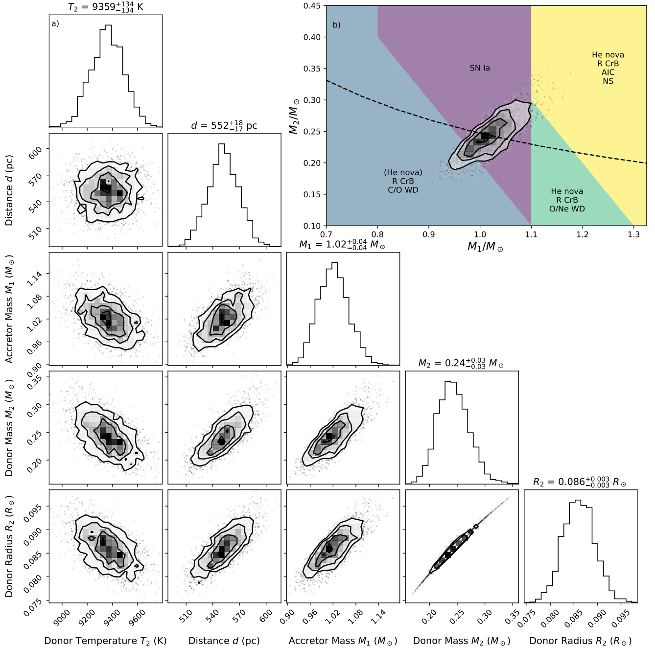
Figure 4. Constraints on the component masses, donor temperature and radius, and distance. (a) Corner plots for the fitting procedure. We simultaneously fit the SED data with the Gaia astrometric constraint and the spectroscopic radial velocity constraint, but assuming the same density since the donor is filling its Roche lobe. (b) Outcomes of interacting double white dwarf binaries from K. J. Shen (2015), with the posterior distributions of the component masses of ATLAS J1138-5139 and a dashed line of constant chirp mass.
