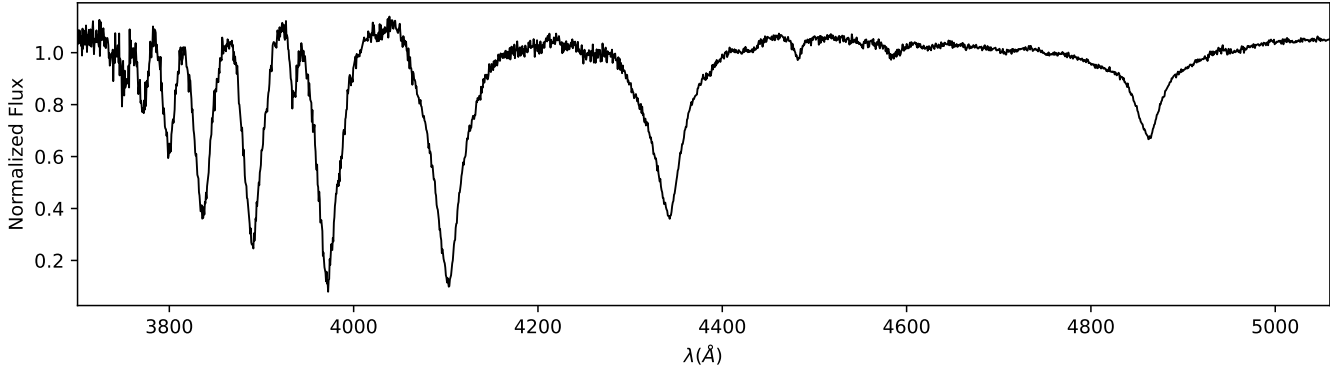
Figure 8. Bluest portion of the coadded MagE spectrum of ATLAS J1138-5139, showing the Balmer series from the white dwarf donor.
