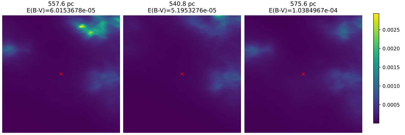
Figure 3. Interstellar dust extinction maps illustrating the extinction along the line of sight to ATLAS J1138-5139 at three distances. The first panel corresponds to the system’s observed distance d = 557 pc, the second panel shows the extinction at d - \sigma_{d,\text{lower}} = 541 pc, and the third panel represents d + \sigma_{d,\text{upper}} = 576 pc, where \sigma_d is the uncertainty in the distance measurement. The location of the system is marked with a red “X” in all panels. The values of E(B - V) are negligible across all distances.
