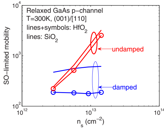
FIG. 2. (Color online) Effect of Landau damping on SO-limited hole mobility in a relaxed GaAs p-channel of an MOS system with an SiO 2 or an HfO 2 gate insulator.
