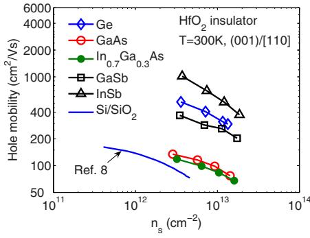
FIG. 11. (Color online) As in Fig. 10 but with HfO 2 insulator.
