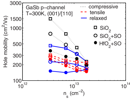
FIG. 7. (Color online) As in Fig. 5, but for GaSb channels.
