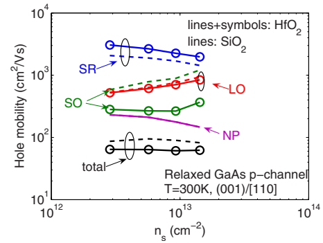
FIG. 4. (Color online) Hole mobility components in a relaxed GaAs p-channel with SiO 2 and HfO 2 insulators.
