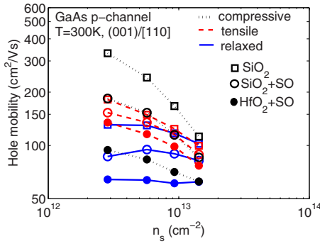
FIG. 6. (Color online) As in Fig. 5, but for GaAs channels.
