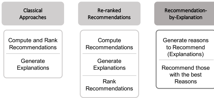
Fig. 2: Role of explanations in producing recommendations.
