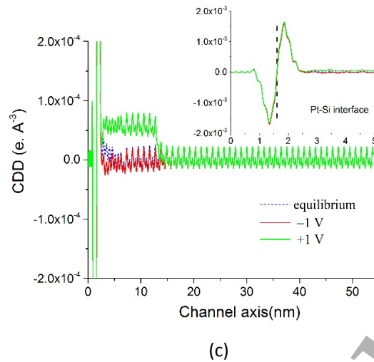
Fig. 4. Planar average of the charge difference density (CDD) for (a) semimetal/semiconductor (thick/thin) \alpha -Sn, (b) Ag/Si, and (c) Pt/Si junctions for applied gate voltages of -1 V, 0 V, and +1 V. Insets show details of the CDD at the interfaces and with the vertical dashed lines indicate the metallurgical junction location.
