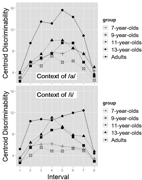
FIG. 5. Mean /s/-/ʃ/ centroid discriminability values for each age group at every interval, in the two vowel contexts (the context of /a/ in the top panel, the context of /i/ in the bottom panel).
