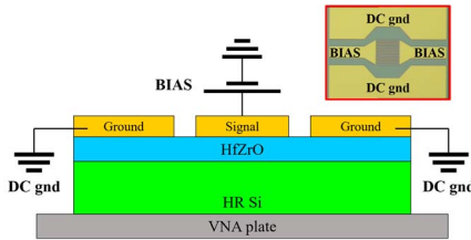
Fig. 3. Schematic representation of the DC/MW measurement setup (in the inset, an optical picture with the top-view of the HfZrO-based IDC is shown).
