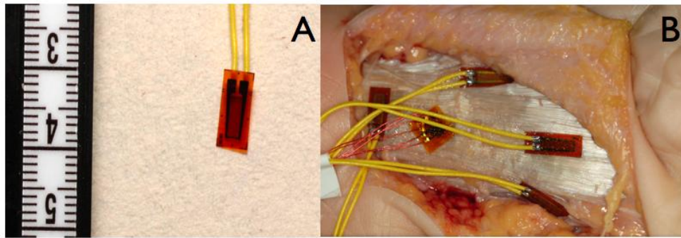
Figure 5.2: A: 10mm, 120Ohm foil-type microstrain gauges (BCM Sensor Technologies, Antwerp, Belgium) B: Microstrain gauge external fixation to fascia with gauge specific cyanoacrylate adhesive (TML, Tokyo, Japan).
