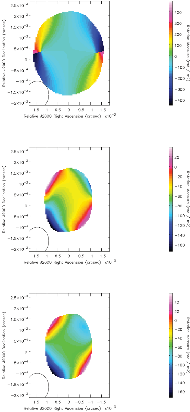
Figure A6. Results of Monte Carlo simulations using model core-jet sources with oppositely directed transverse RM gradients in the core region and inner jet. The intrinsic width of the jet (RM gradient) is 0.35 mas. The convolving beam ( 1.28 \text{ mas} \times 1.06 \text{ mas} in \text{PA} = -0^\circ:84 ) is shown in the lower left-hand corner of each panel. The top panel shows the RM image obtained by processing the model data as usual, but without adding random noise or EVPA calibration uncertainty; pixels with RM uncertainties exceeding 10 \text{ rad m}^{-2} were blanked. The remaining two panels show two examples of the 200 individual RM images obtained during the simulations; pixels with RM uncertainties exceeding 80 \text{ rad m}^{-2} were blanked.
