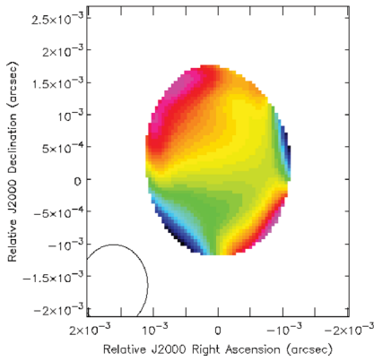
Figure A8. Same as Fig. A6 for a core-jet source with the same length but an intrinsic jet width of 0.10 mas.
