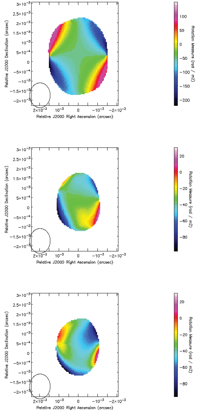
Figure A7. Same as Fig. A6 for a core-jet source with the same length but an intrinsic jet width of 0.20 mas.
