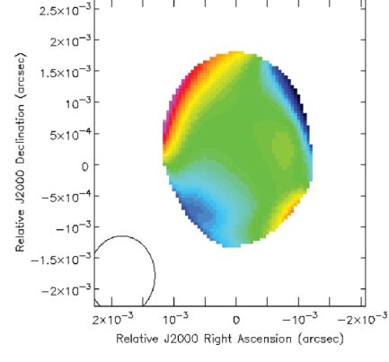
Figure A9. Same as Fig. A6 for a core-jet source with the same length but an intrinsic jet width of 0.05 mas.
