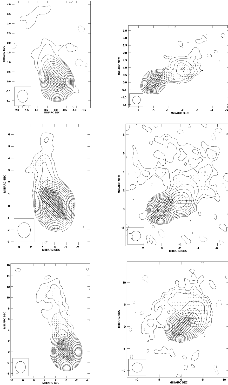
Figure 1. VLBA I maps for 0716+714 (left) and 1749+701 (right) with polarization sticks superimposed, at 15.4 GHz (top), 7.9 GHz (middle) and 4.6 GHz (bottom), corrected for integrated Faraday Rotation. The maps of 0716+714 have peaks of 1.0, 1.3 and 1.5 Jy beam -1 and bottom contours of 0.7, 0.8 and 0.9 mJy beam -1 ; the maps of 1749+701 have peaks of 0.5, 0.4 and 0.3 Jy beam -1 and bottom contours of 0.6m, 0.5 and 1.7 mJy beam -1 .
