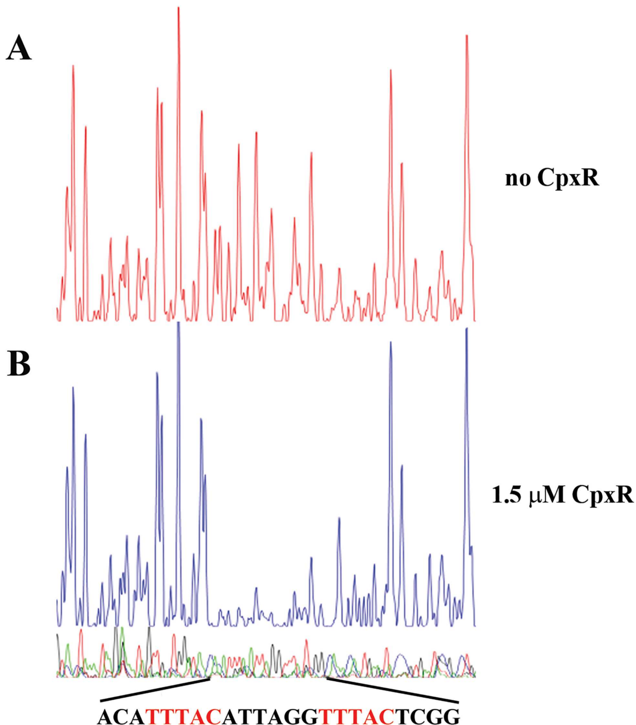
Fig 2. Direct binding of CpxR to the promoter region of mexA in vitro . DNase I footprinting assays of the mexA promoter DNA fragment were performed in the absence (A) and presence (B) of purified CpxR. The FAM-labelled 322-bp DNA fragments (50 nM) pre-incubated in the absence or presence of 1.5 μM phosphorylated CpxR were subjected to DNase I digestion and fragment length analysis. The fluorescence signal of the labelled DNA fragments is plotted against the sequence of the fragment. The protected region bound by CpxR is shown with the conserved binding motif in red.
