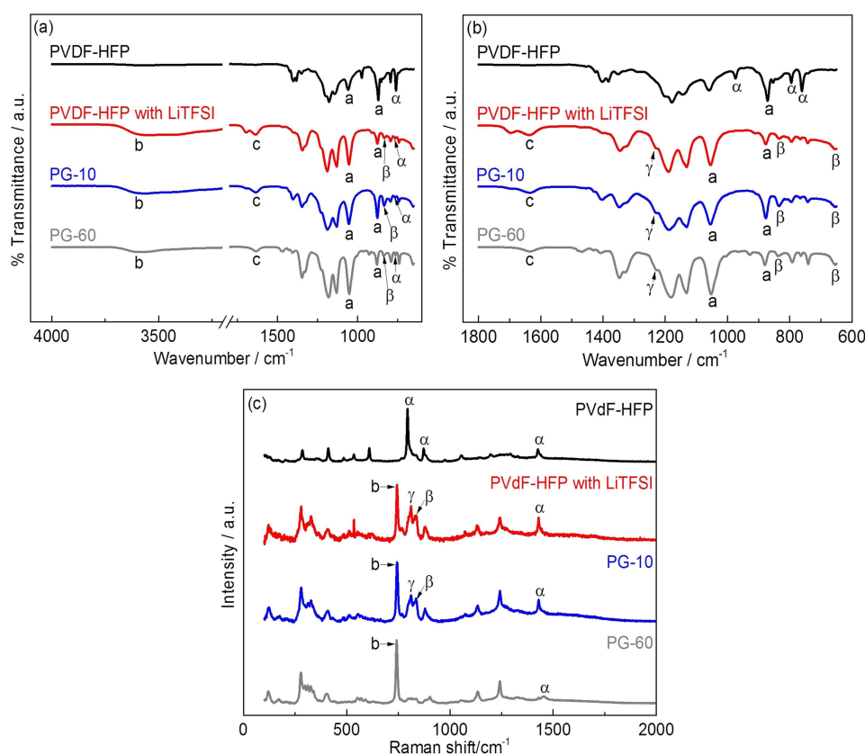
Figure 3. Room temperature FT-IR spectra of PVDF-HFP, PVDF-HFP with LiTFSI, PG-10 and PG-60, (a) displaying the range 4000 cm -1 to 650 cm -1 , (b) displaying the range 1800 cm -1 to 650 cm -1 , (c) room temperature Raman spectra of PVDF-HFP, PVDF-HFP with LiTFSI, PG-10 and PG-60.
