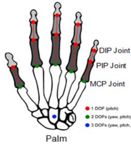
Fig. 8. Degrees of freedom of hand.
