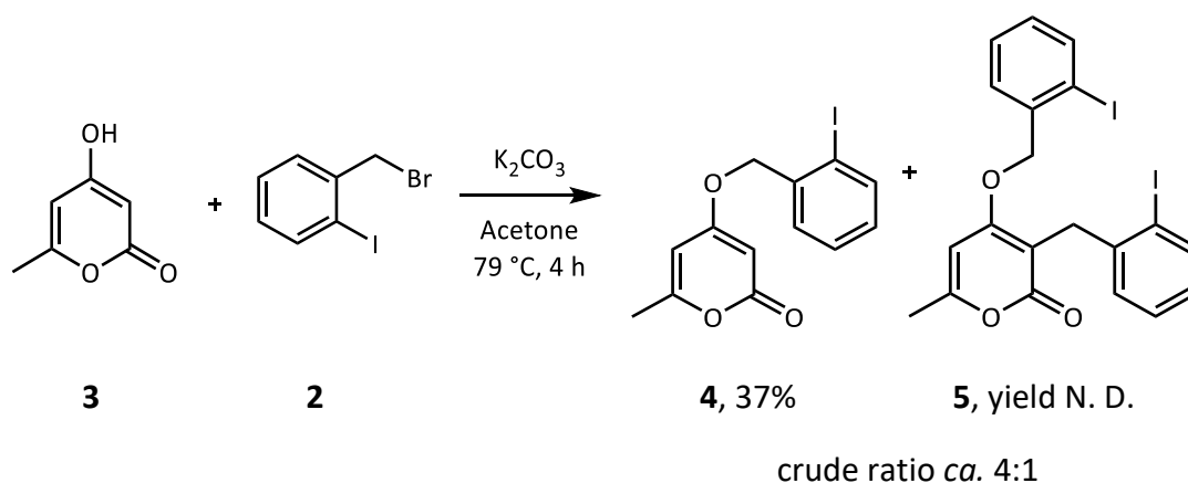
Scheme 2.3. Benzylation of 4-hydroxy-2-pyrone 3 .
