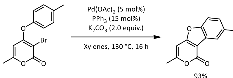
Scheme 1.9. Intramolecular direct arylation of 3-bromo-2-pyrone.
