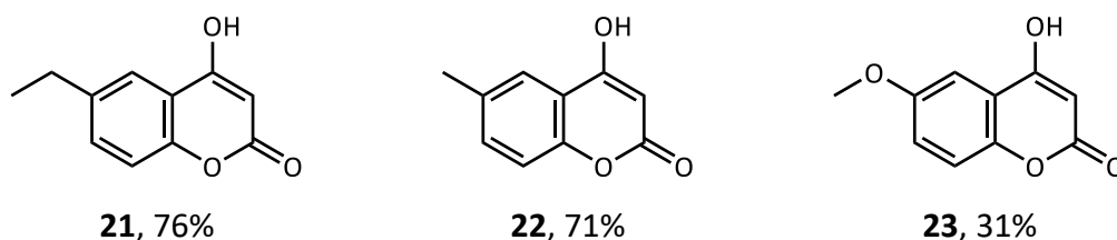
Scheme 2.11. Synthesis of substituted 4-hydroxy-2-coumarins 21-23 .
