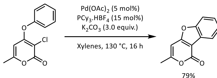
Scheme 1.10. Intramolecular direct arylation of 3-chloro-2-pyrones.
