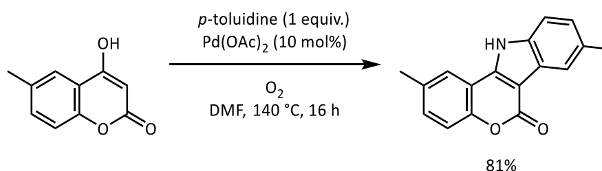
Scheme 1.39. Cross-dehydrogenative coupling of 4-anilino-2-coumarins.
