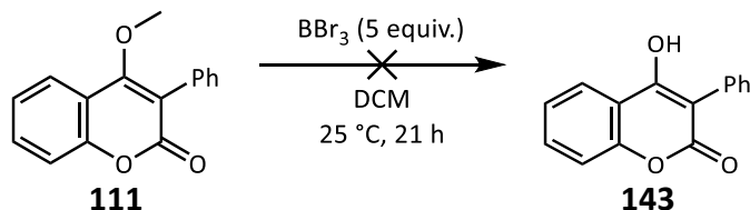
Scheme 3.24. Attempt to demethylate 111 with \text{BBr}_3 .
