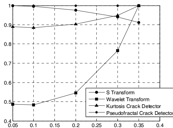
Figure 5. Comparison of methods for damage extent calibration
