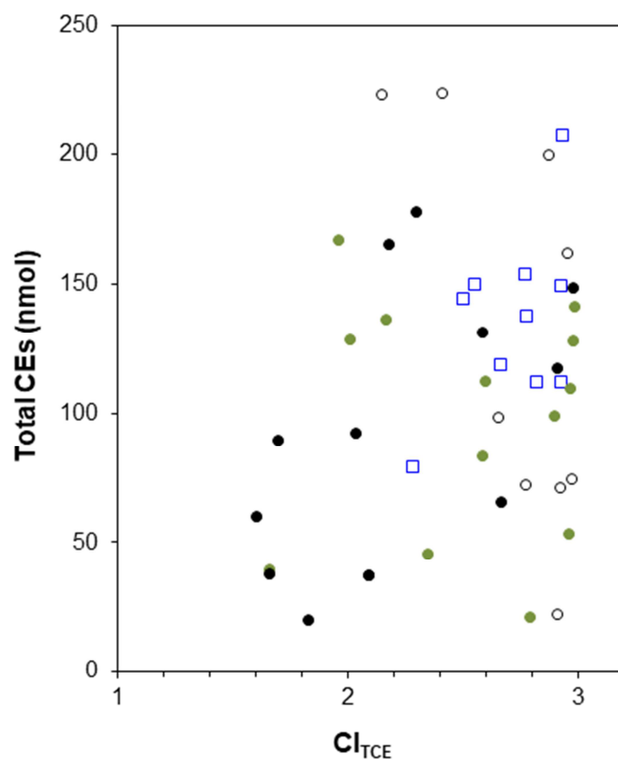
Figure 5: Relationship between total pore water CEs (in nmol) and the chlorine index of TCE ( CI_{TCE} ) in all riverbed samples where CI_{TCE} = <3 . Blue squares (reach-scale mini-piezometer samples); open circles (upstream PW samples); green circles (mid-point PW samples); black circles (downstream PW samples).
