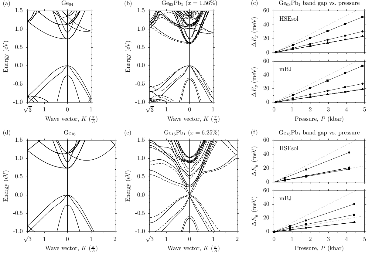
FIGURE 5.2: Band structure of (a) \text{Ge}_{64} ( 2 \times 2 \times 2 SC), (b) \text{Ge}_{63}\text{Pb}_1 ( x = 1.56\% ), (d) \text{Ge}_{16} ( 2 \times 2 \times 2 FCC), and (e) \text{Ge}_{15}\text{Pb}_1 ( x = 6.25\% ), calculated via DFT using the HSEsol (solid lines) and mBJ (dashed lines) XC functionals. (c) Calculated change in band gap \Delta E_g with applied hydrostatic pressure P for the \text{Ge}_{63}\text{Pb}_1 supercell of (b), calculated using the HSEsol (upper panel) and mBJ (lower panel) XC functionals. Band gaps are calculated between the VB edge and the first (circles), second, third and fourth (triangles), and fifth (squares) lowest energy CB states. (f) As in (c), but for the \text{Ge}_{15}\text{Pb}_1 supercell of (e). The lower (upper) dashed grey line in (c) and (f) denotes the variation with pressure of the indirect L_{6c}-\Gamma_{8v} (direct \Gamma_{7c}-\Gamma_{8v} ) band gap of Ge.
