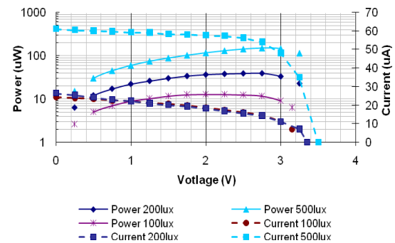
Fig.5 The I-V and P-V characteristics of the Schott Solar's ASI2Oi05/055/014JF
