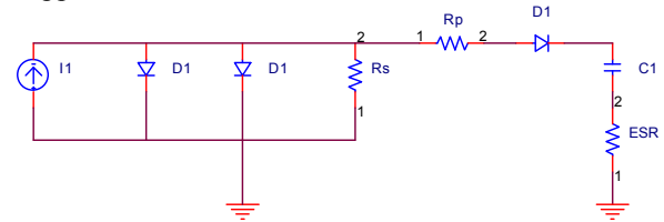
Fig. 7 System Simulation Schematics
