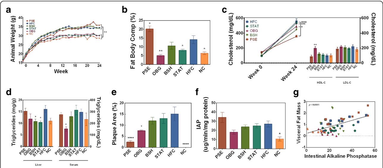
Fig. 1 Effect of cardiovascular disease interventions on adiposity, cholesterol and lipid profile, atherogenesis, and inflammation. a Animal weight gain over the 24-week intervention period. b Percentage fat of animals prior to cull. c Serum total and HDL and LDL cholesterol evolution over 24-week period. d Liver and serum triglyceride levels following intervention. e Aortic plaque as percentage of total area. f Intestinal alkaline phosphatase (IAP) activity in jejunum tissue. g Positive correlation between visceral fat mass and IAP activity, with confidence bands displayed by dashed lines. * ( p < 0.05 ), ** ( p < 0.01 ), and *** ( p < 0.001 ) represent significant differences when compared against HFC in one-way ANOVA. Plots depict significant differences and plots depict individual replicates with mean and SEM
