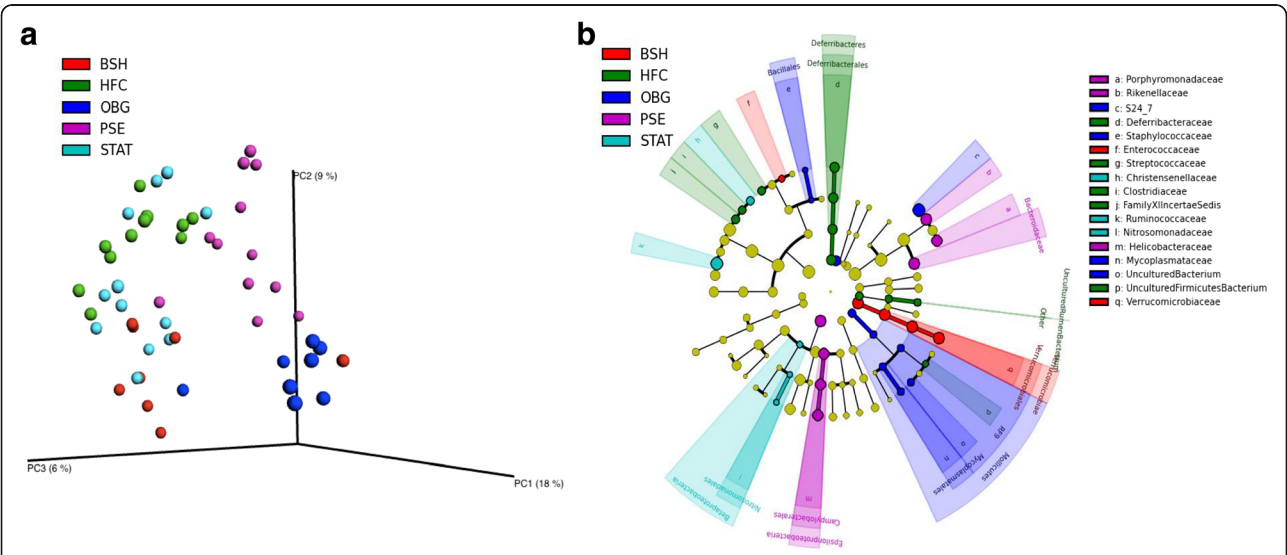
Fig. 2 Effect of cardiovascular disease interventions on the microbiome composition. Unweighted unifrac principle coordinate analysis (PCoA) plots ( a ), with linear discriminant analysis (LDA) effect size (LEfSe) representation of taxa associated with HFC and each intervention ( b )
