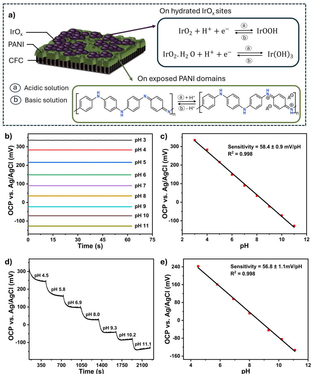
Fig. 4 (a) Schematic illustration of the pH sensing mechanism; (b) open circuit potential response of the electrode in standard buffer solutions from pH 3 to 11 and (c) its corresponding calibration curve; (d) continuous OCP response recorded in Britton–Robinson buffer while the pH was adjusted from 4.5 to 11.1 by adding 1 M NaOH without removing or washing the sensor and (e) corresponding calibration curve extracted from the continuous pH response measurement.
