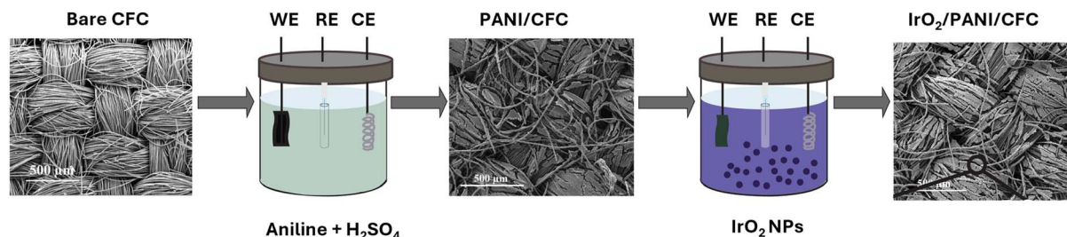
Scheme 1 Schematic illustration of the fabrication route of the IrO 2 /PANI/CFC pH sensor.
