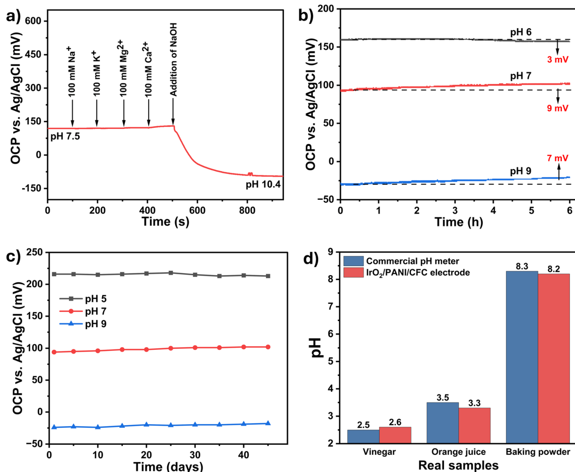
Fig. 5 (a) Interference study in the presence of common cations, including \text{Na}^+ , \text{K}^+ , \text{Mg}^{2+} and \text{Ca}^{2+} followed by pH adjustment using NaOH; (b) short-term OCP drift response recorded at fixed pH values during 6 hours continuous measurement; (c) long-term stability of the electrode measured at pH 5, 7 and 9 over 45 days. (d) Real sample pH analysis of vinegar, orange juice and baking powder solution compared with a commercial pH meter.
