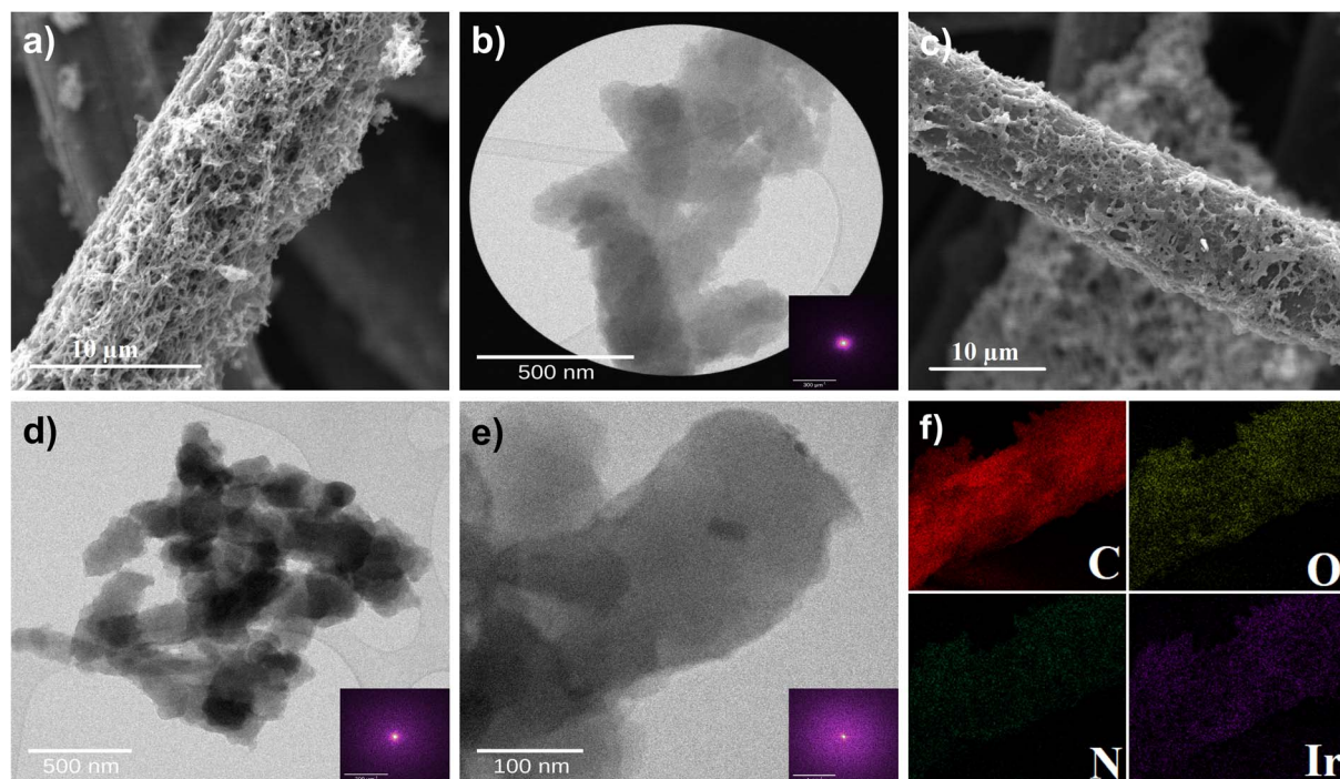
Fig. 2 (a) SEM and (b) TEM images of PANI/CFC; (c) SEM, (d) TEM and (e) high-magnification TEM image of \text{IrO}_2 /PANI/CFC with FFT inset of \text{IrO}_2 /PANI/CFC; (f) EDX elemental maps of \text{IrO}_2 /PANI/CFC showing C, N, O, and Ir distributions, respectively.
