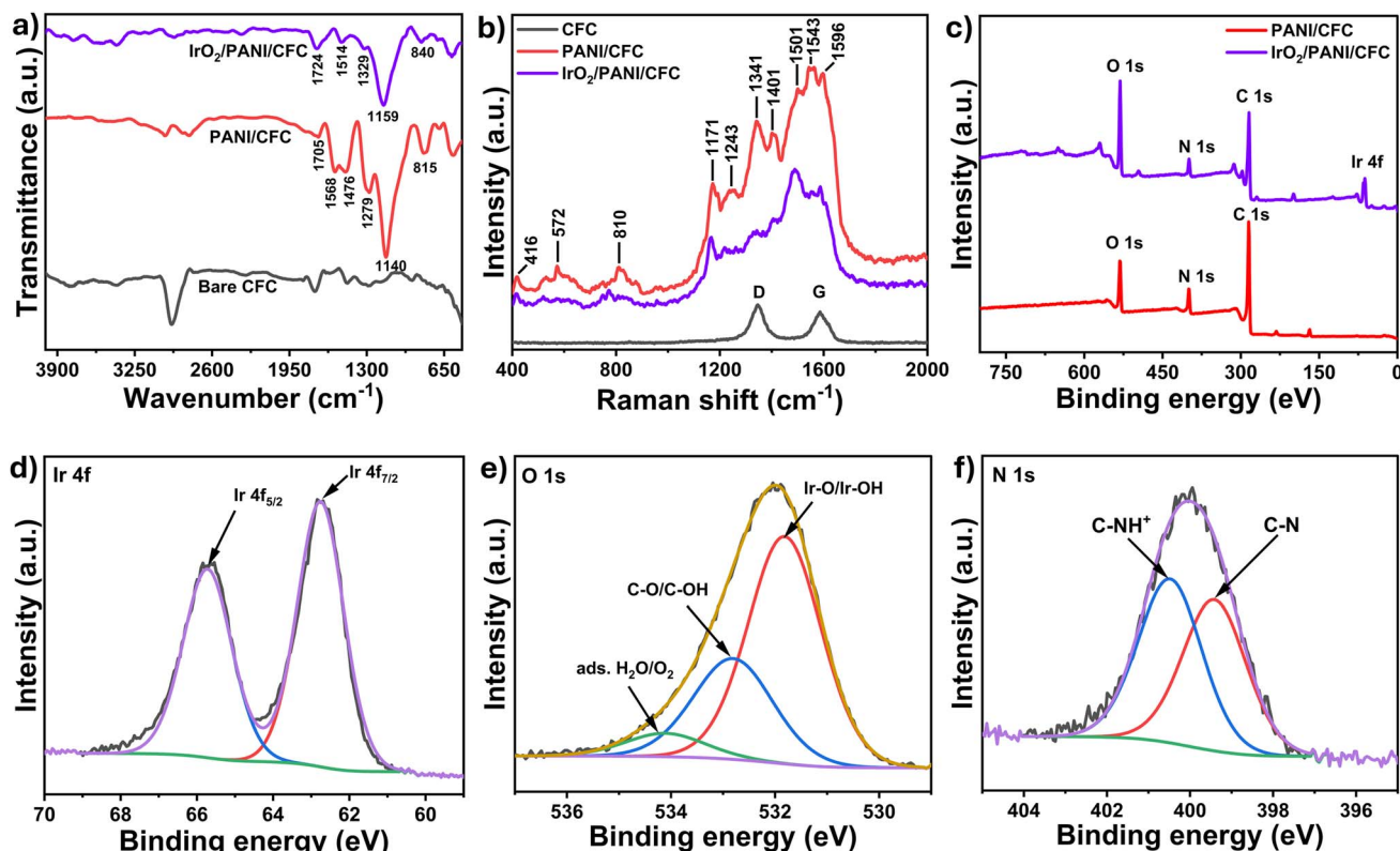
Fig. 3 (a) FTIR spectra of CFC, PANI/CFC, and IrO 2 /PANI/CFC; (b) Raman spectra of CFC, PANI/CFC, and IrO 2 /PANI/CFC; (c) XPS survey spectra of PANI/CFC and IrO 2 /PANI/CFC; high-resolution XPS spectrum of IrO 2 /PANI/CFC: (d) Ir 4f, (e) O 1s, (f) N 1s.
