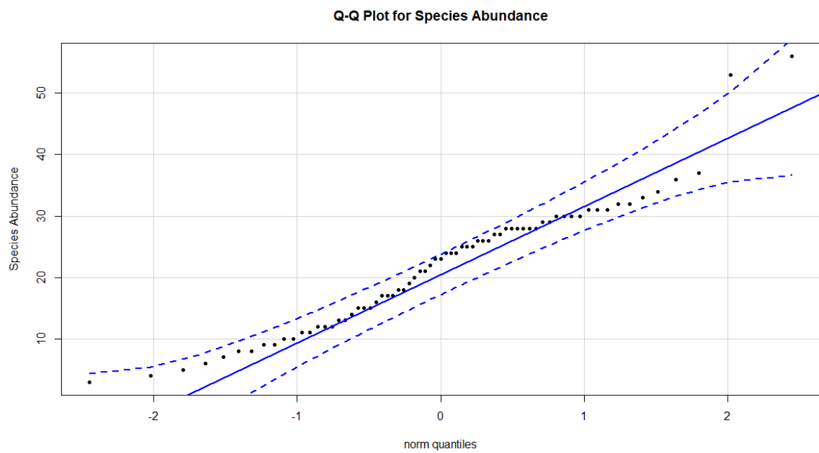
Fig.16: The species abundance QQ plot, showing a relatively Gaussian distribution.
