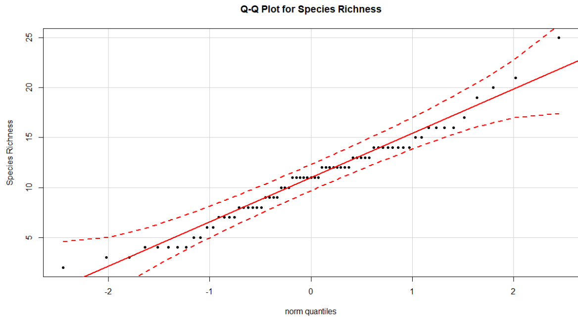
Fig.15: The species richness QQ plot, displaying a Gaussian distribution.
