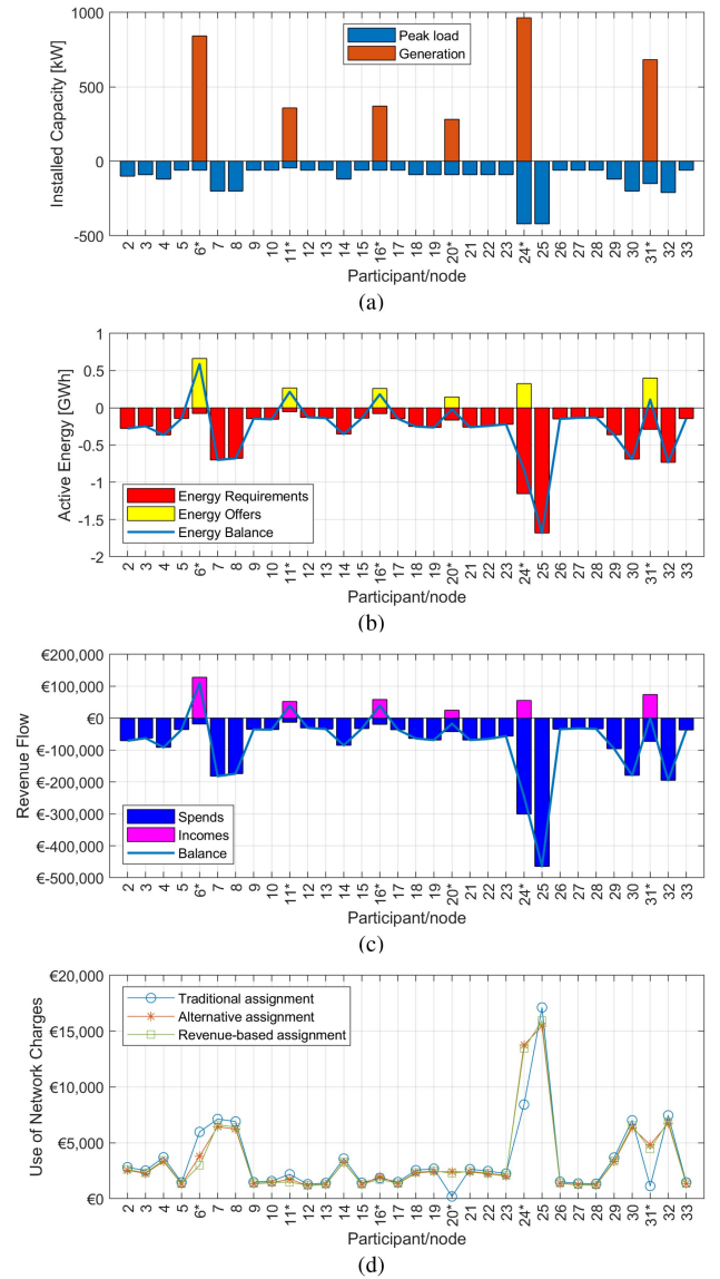
Fig. 4. Detailed results for DER allocation method [17] considering ToU and electrical distance over the course of the studied year. (*) Participant nodes with DER. (a) Installed DER and peak load, (b) energy balance resulting from PF simulations, (c) economic balance, and (d) assignments of charges.
