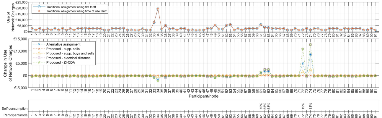
Fig. 7. Change in use of network charges assigned to participant nodes in the IEEE 123-bus network using DER allocations in [21].
