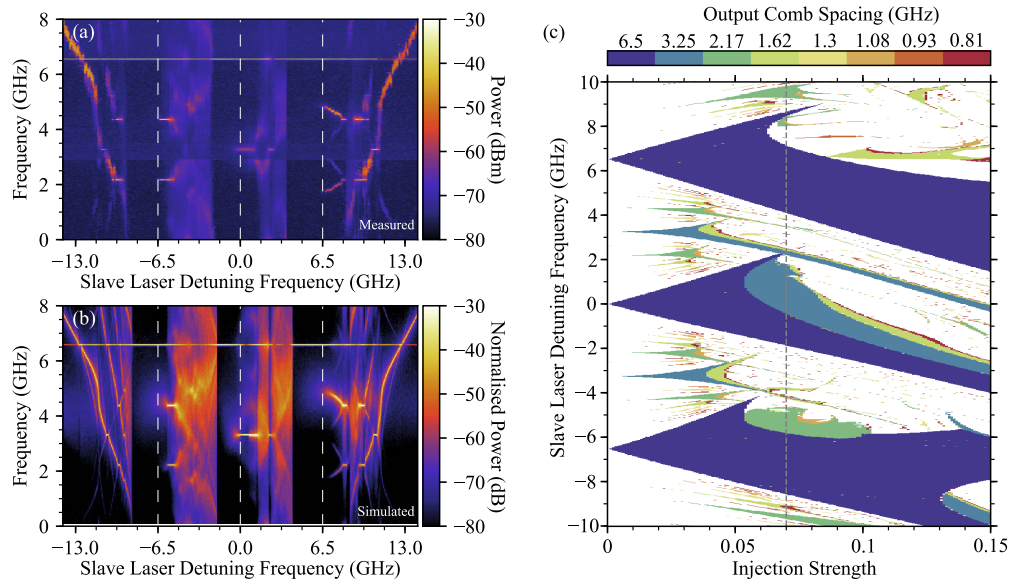
Fig. 7. (a) Intensity plot showing the electrical spectra measured as the frequency of a single mode slave laser was swept across the injected 6.5 GHz optical comb. The optical comb had a power of -5.0 dBm, and the slave laser was initially biased at 1.75 times threshold current, with -4.4 dBm coupled to the lensed fibre. The vertical dashed white lines show the parameter values where the free-running laser frequency is resonant to one of the optical comb lines. (b) Corresponding simulated experiment for the parameters in (a). (c) Two dimensional map of the parameter space spanned by detuning and injected power, showing the output comb frequency spacing, calculated with J = 1.75J_{th} and \Delta_{comb} = 6.5 GHz. The vertical dotted line indicates the injection strength used in (b). White regions indicate unlocked states.
