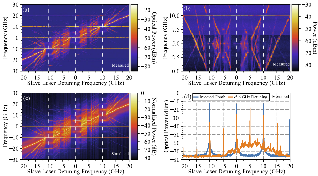
Fig. 4. Experimental and theoretical results from a frequency detuning sweep. In the experimental results, the slave laser was initially biased at 1.75 times threshold current with free-running power -4.5 dBm, and was injected by 3 line comb of total power -7 dBm, with spacing \Delta_{\text{comb}} = 10 GHz. The slave laser's temperature was varied to perform the frequency detuning sweep, and the vertical dashed white lines show where the free-running laser frequency is resonant to one of the optical comb lines. (a) Intensity plot of measured optical spectra as the slave laser was tuned across the injected optical comb. The frequency axis has been scaled such that 0 GHz coincides with the centre comb line. (b) Electrical power spectra for the corresponding frequency sweep in (a). (c) Intensity plot of simulated optical spectra with K = 0.06 , for the same parameters as in (a). (d) Comparison between the optical spectra of the injected comb, and the output comb as the slave is frequency locked between the optical comb lines (at a detuning of -5.6 GHz).
