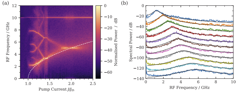
Fig. 3. (a) Calculated RF spectrum of a slave laser under optical injection from a 10 GHz comb, as the pump current of the slave is swept. The dashed white line indicates the frequency of the free-running ROs. The injection strength of K = 0.06 was fixed. (b) Measured free-running ROs of the slave laser from 55 mA to 120 mA, in steps of 5 mA up until 90 mA and steps of 10 mA thereafter, offset vertically from top to bottom by -10 dB for clarity. Solid black lines indicate fits from which we determined parameter values for our model.
