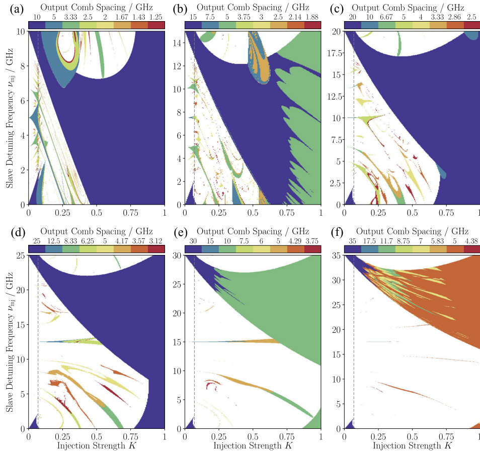
Fig. 8. Two dimensional maps of the parameter space spanned by detuning and injected power, which show the output frequency spacing of the slave laser, calculated with J = 1.82J_{th} (corresponding to an RO frequency of 4.375 GHz). The comb spacings used were (a) 10 GHz, (b) 15 GHz, (c) 20 GHz, (d) 25 GHz, (e) 30 GHz, and (f) 35 GHz. White regions indicate unlocked states.
