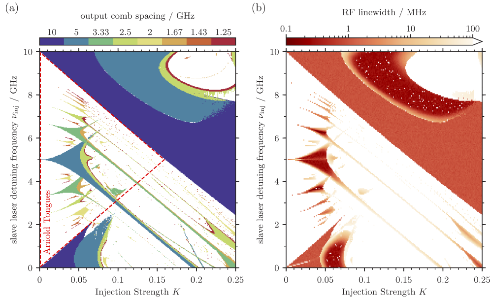
Fig. 5. Two dimensional maps of the parameter space spanned by detuning and injected power, calculated with J = 1.82J_{th} and \Delta_{comb} = 10 GHz. (a) Map of the output comb frequency spacing. White regions indicate unlocked states. The triangular region enclosed within the dashed lines shows the parameter region used to calculate the relative size of the harmonic locking areas in Fig. 6. (b) RF linewidth of the dominant harmonic's beat note, over the same parameter space as in (a).
