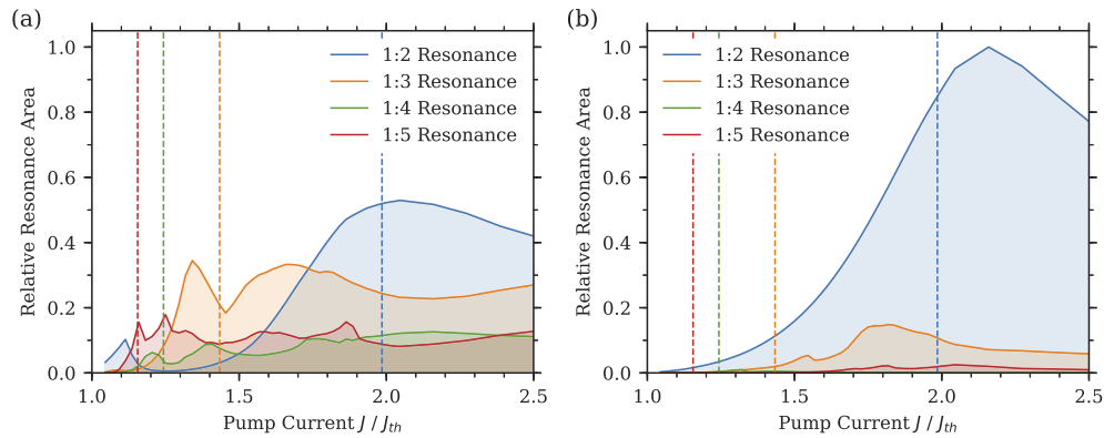
Fig. 6. Plots showing the relative size of the Arnold's resonances as a function of slave laser pump current, for (a) \alpha = 3 , and (b) \alpha = 0 . For each current, a two dimensional map over injection strength and detuning was calculated as in Fig. 5 with \Delta_{\text{comb}} = 10 GHz, and only the area contained in each resonant Arnold's tongue was counted. The vertical dotted lines indicate the pump currents at which the free-running RO frequency matches that of a resonance. Animations showing the two dimensional maps used to calculate the above results are presented in the supplementary material submitted with this manuscript (see Visualization 1 for the \alpha = 3 case, and Visualization 2 for the \alpha = 0 case).
