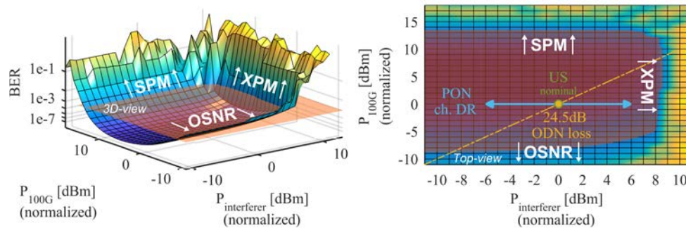
Fig. 8. Upstream BER of the tree architecture as a function of the normalized OOK and 100G signal powers. The contour corresponding to the FEC threshold of 1.1E-3 is clearly visible from the top-view. The straight line visible from the top-view represents the ODN loss.
