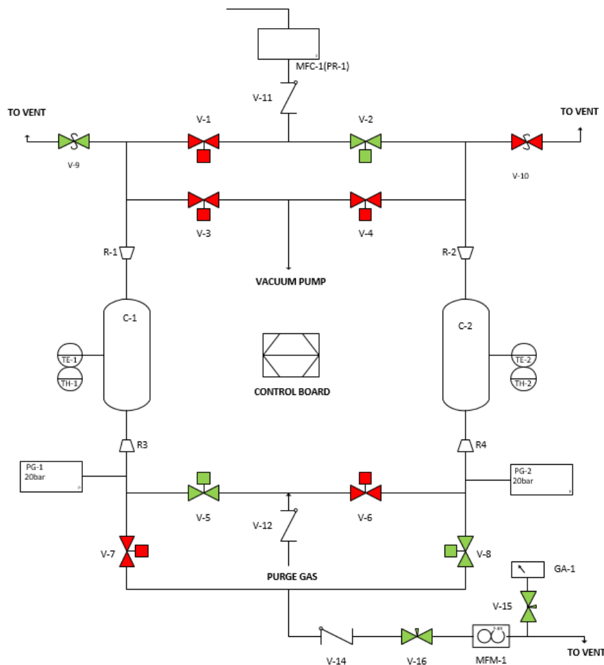
Figure 28 Operation 4 Valve control scheme
