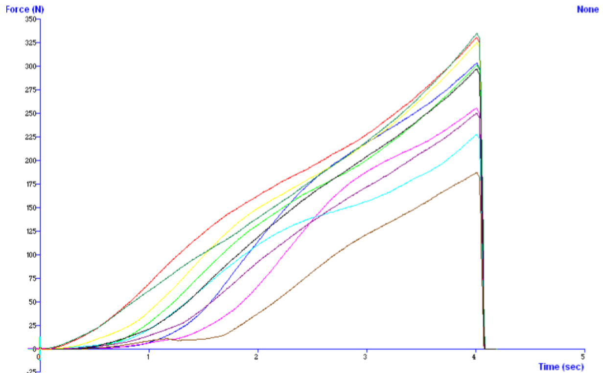
Figure 67 Force v Time graph (compressive strength) for 1mm diameter cylindrical pellets (10 units, Batch 1)
