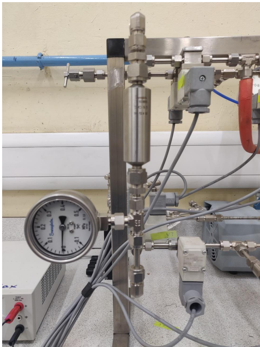
Figure 48 PVSA Sample column C-1 and pressure gauge PG-1
