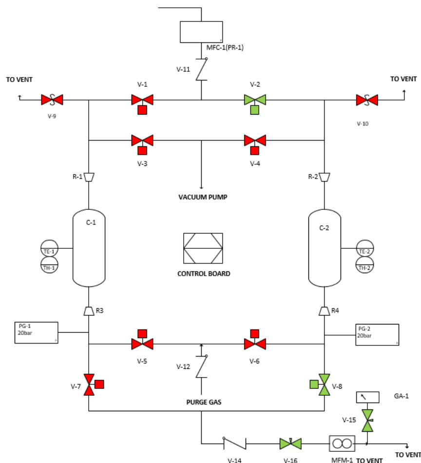
Figure 24 Start-up Control Scheme
