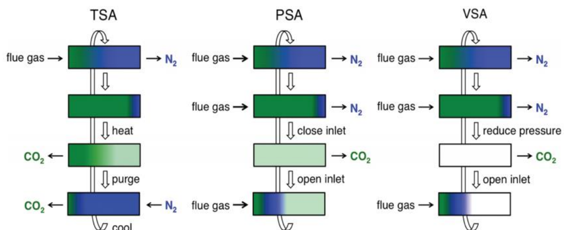
Figure 6 Schematic diagrams of TSA, PSA and VSA processes for regenerating solid adsorbents in fixed-bed columns [29]
