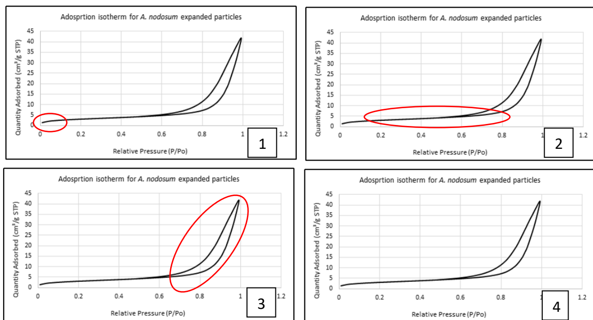
Figure 57 Features of A. nodosum N 2 adsorption isotherm
