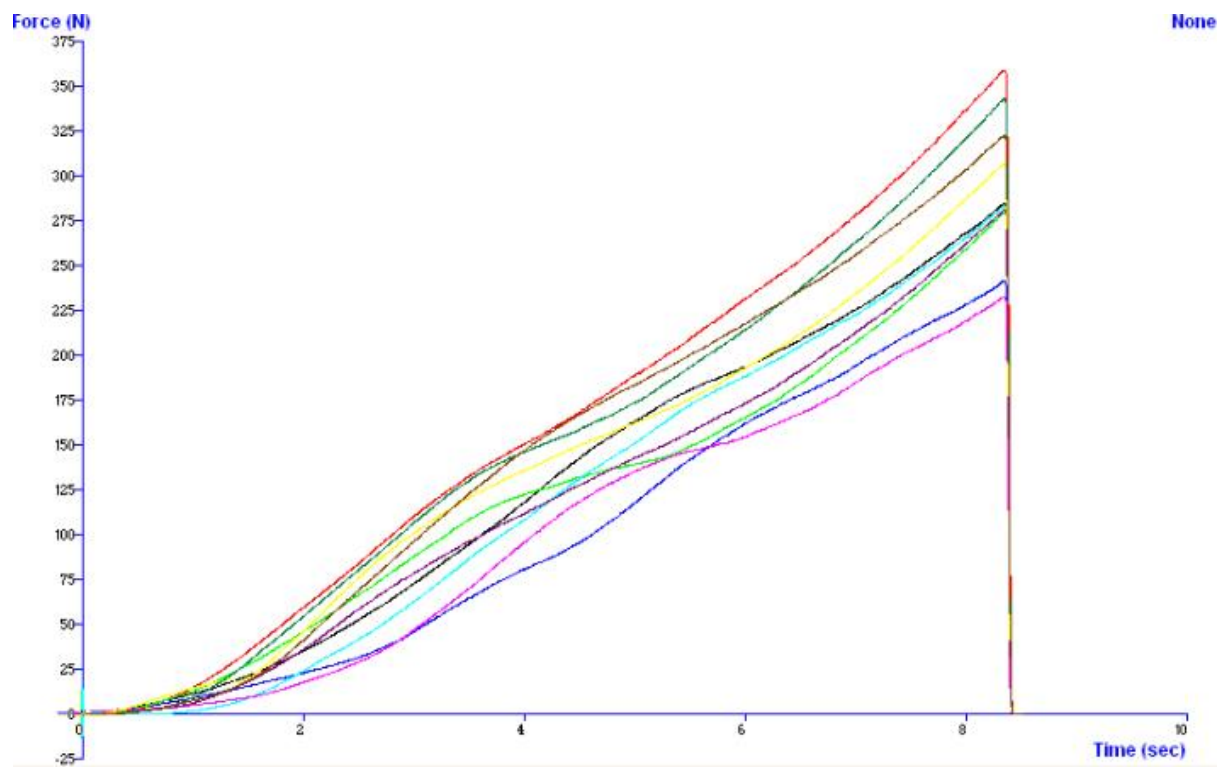
Figure 68 Force v Time graph (compressive strength) for 1mm diameter cylindrical pellets (10 units, Batch 2)
