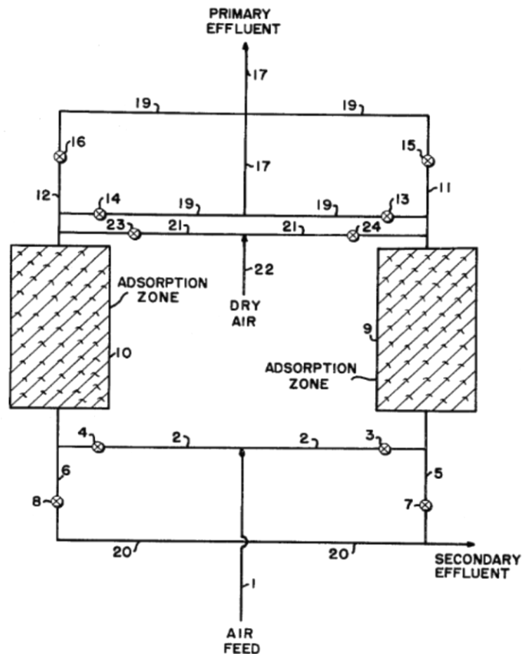
Figure 9 Process patented by Charles Skarstrom [26]
