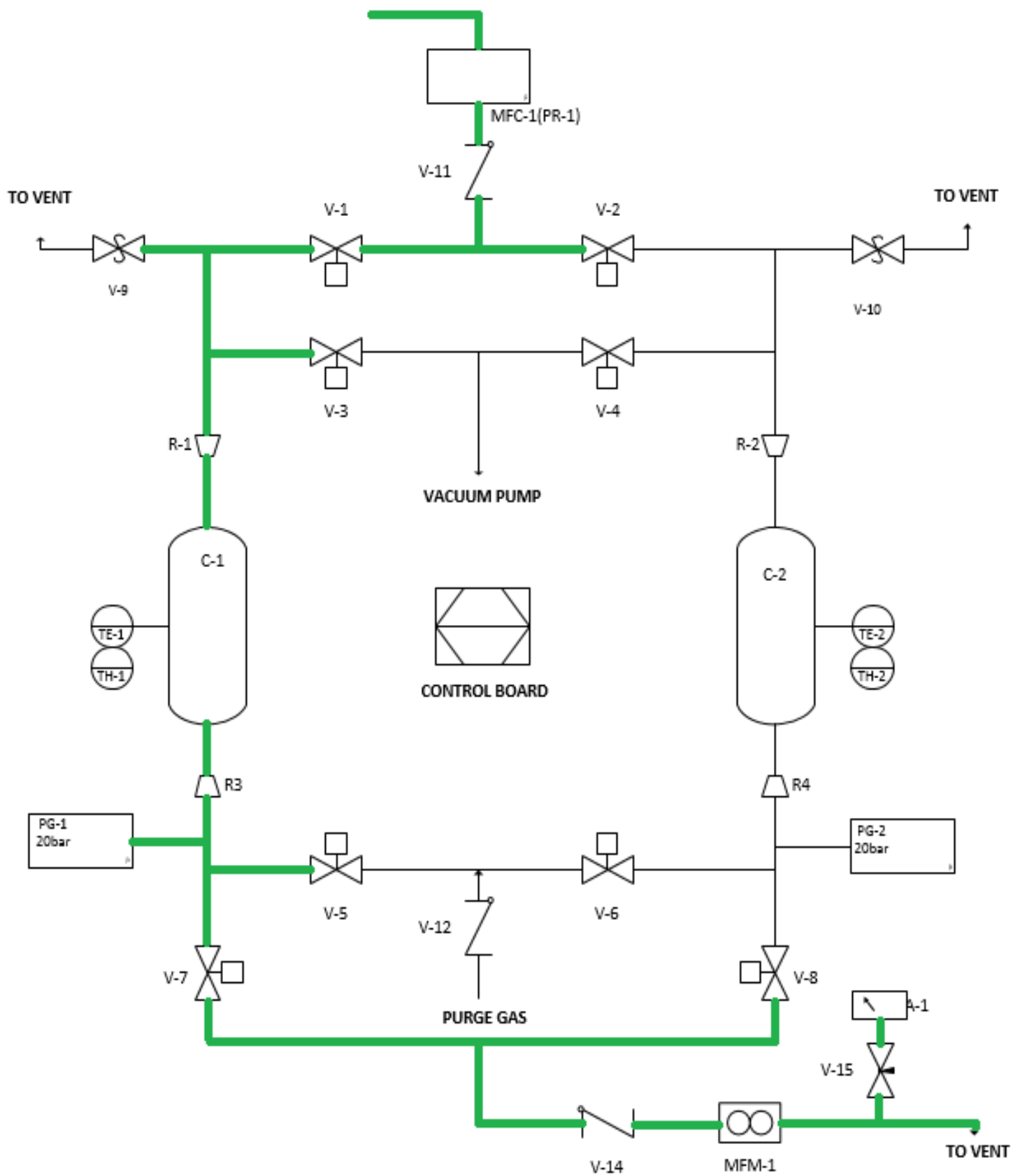
Figure 30 HAZOP Node 1 - Adsorption
