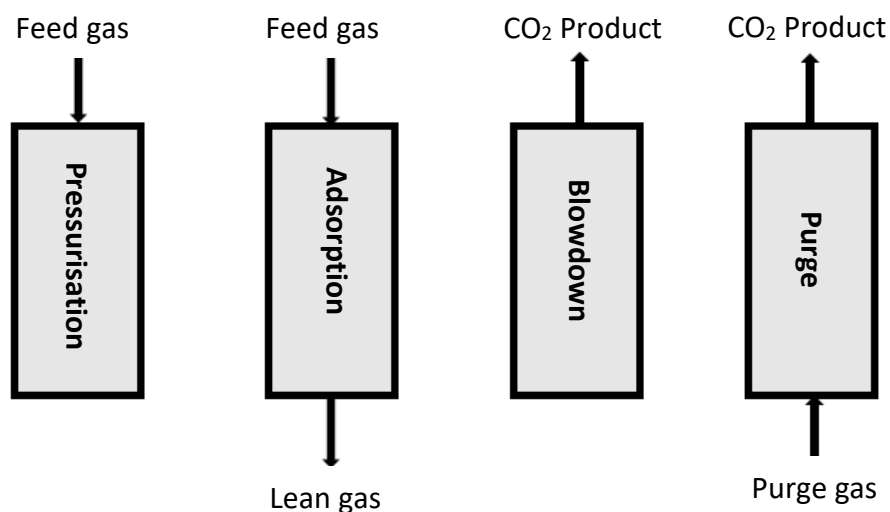
Figure 10 PSA Column operational schematic[38]
