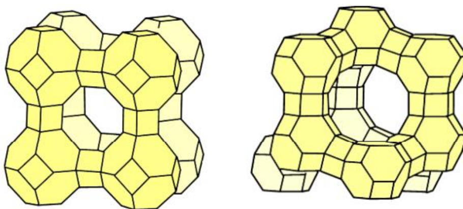
Figure 34 Graphical representation of typical zeolite structures, zeolite A and faujasite [62]
