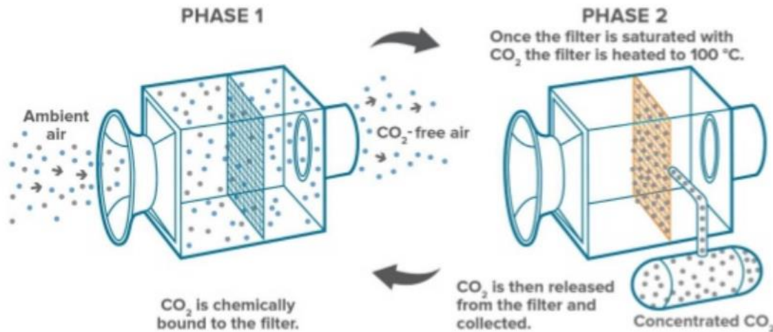
Figure 4 Graphical representation of Climeworks DAC module
