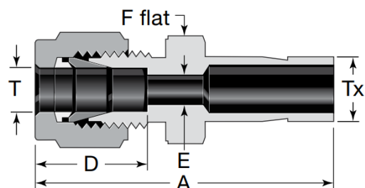
Figure 15 Swagelok Reducer
