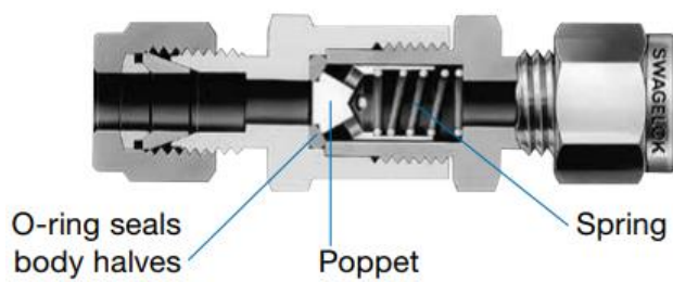
Figure 19 Swagelok poppet check valve
