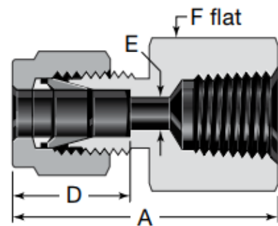
Figure 17 Swagelok NPT Female Connector
