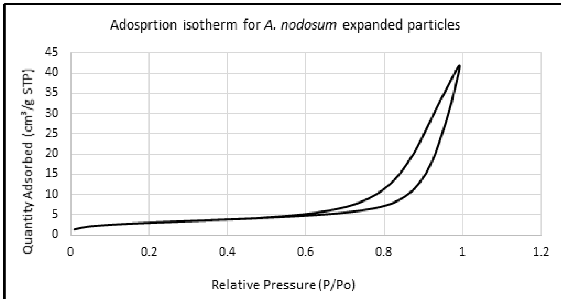
Figure 55 N 2 Adsorption isotherm for A. nodosum expanded particles
