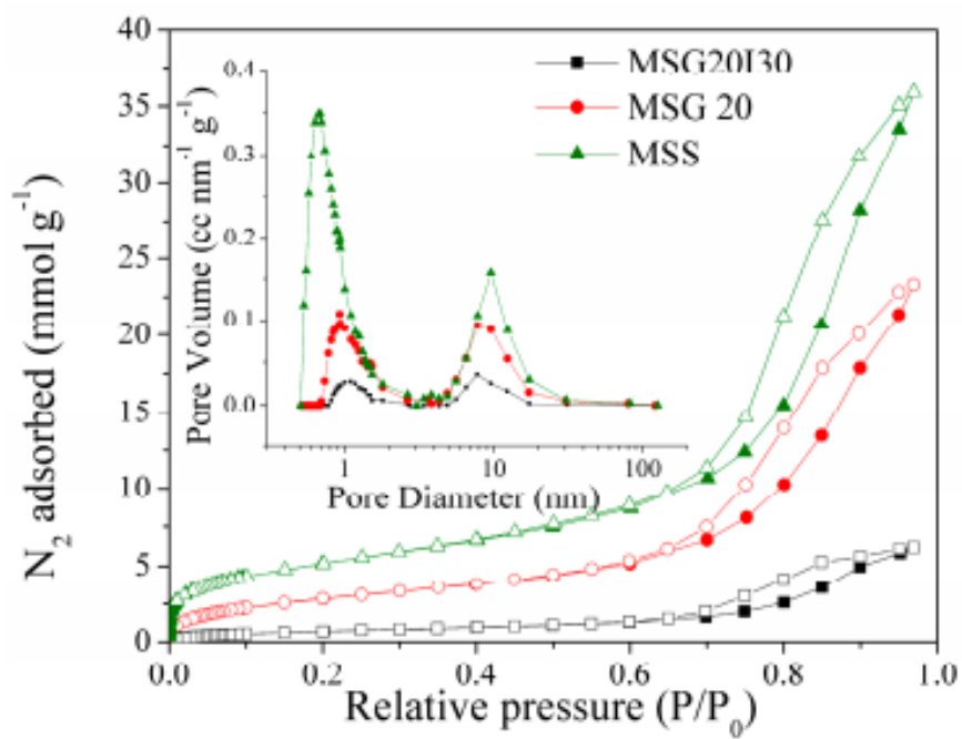
Figure 59 Type IV isotherms of three mesoporous silica-based CO 2 adsorbents [93]
