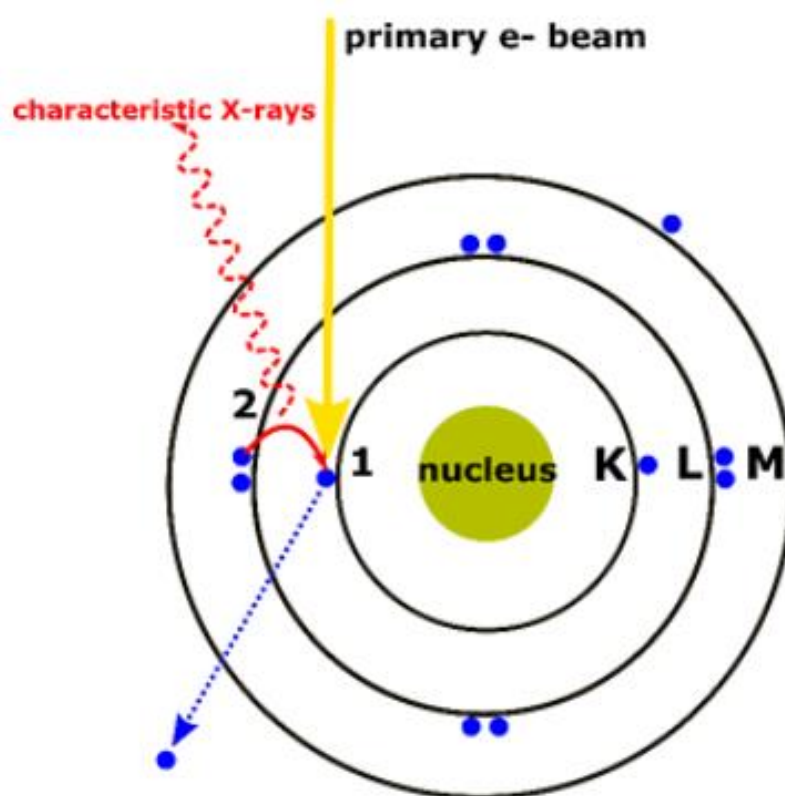
Figure 44 Representation of the process of X-ray emission in an EDX/SEM system[66]
