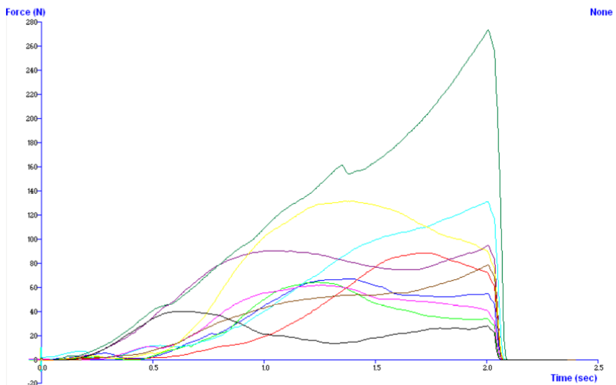
Figure 70 Force v Time graph (compressive strength) for varied agglomerates (10 units, Batch 1)
