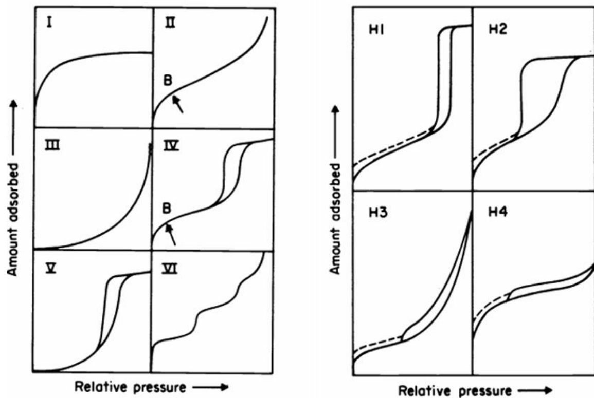
Figure 58 Types of adsorption isotherm and hysteresis loops [90]
