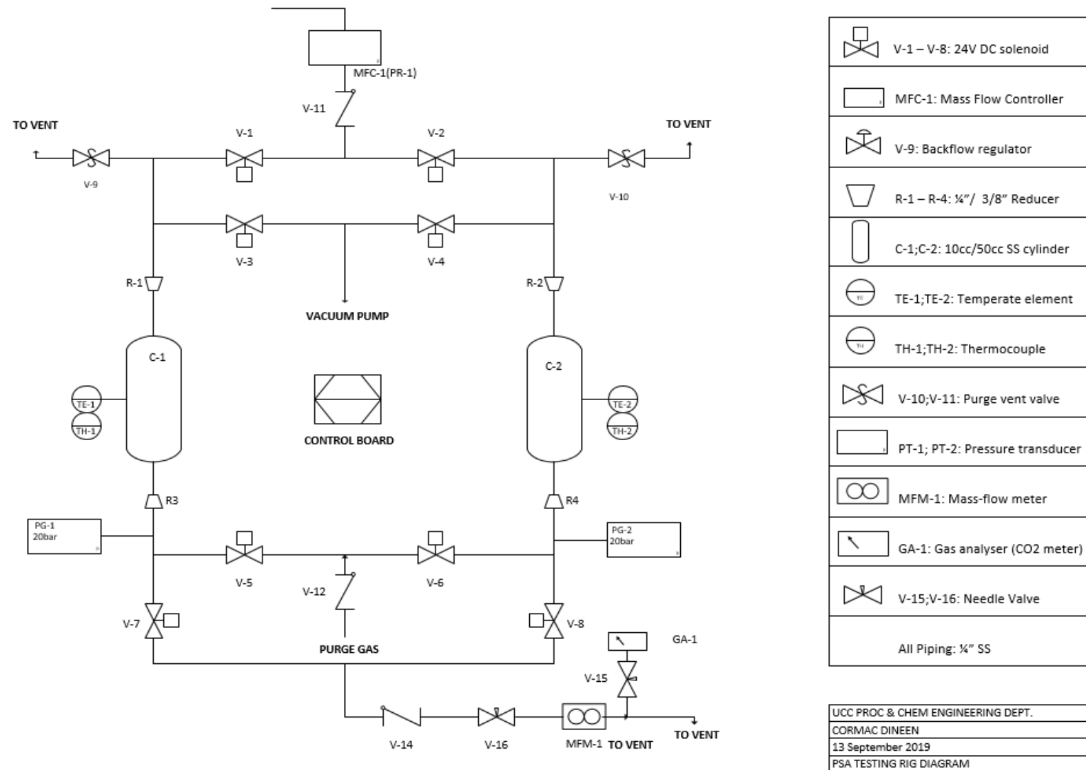
Figure 12 Lab PVSA System PID
