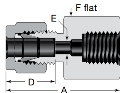
Figure 16 Swagelok Parallel Thread Female Connector
