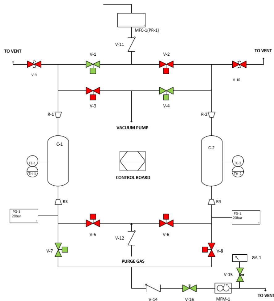
Figure 25 Operation 1 Valve Control Scheme
