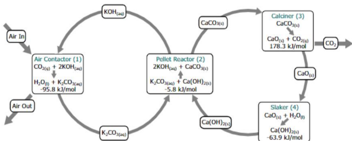
Figure 8 Process Flow diagram of a modified Kraft process for capturing CO 2 from the atmosphere[12]
