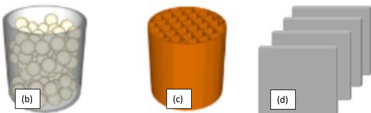
Figure 45 (a) A variety of different solid adsorbent structures [68], (b) granulated or pelletised adsorbent graphical representation, (c) monolithic adsorbent structure graphical representation, (d) laminate adsorbent structure graphical representation [72]
