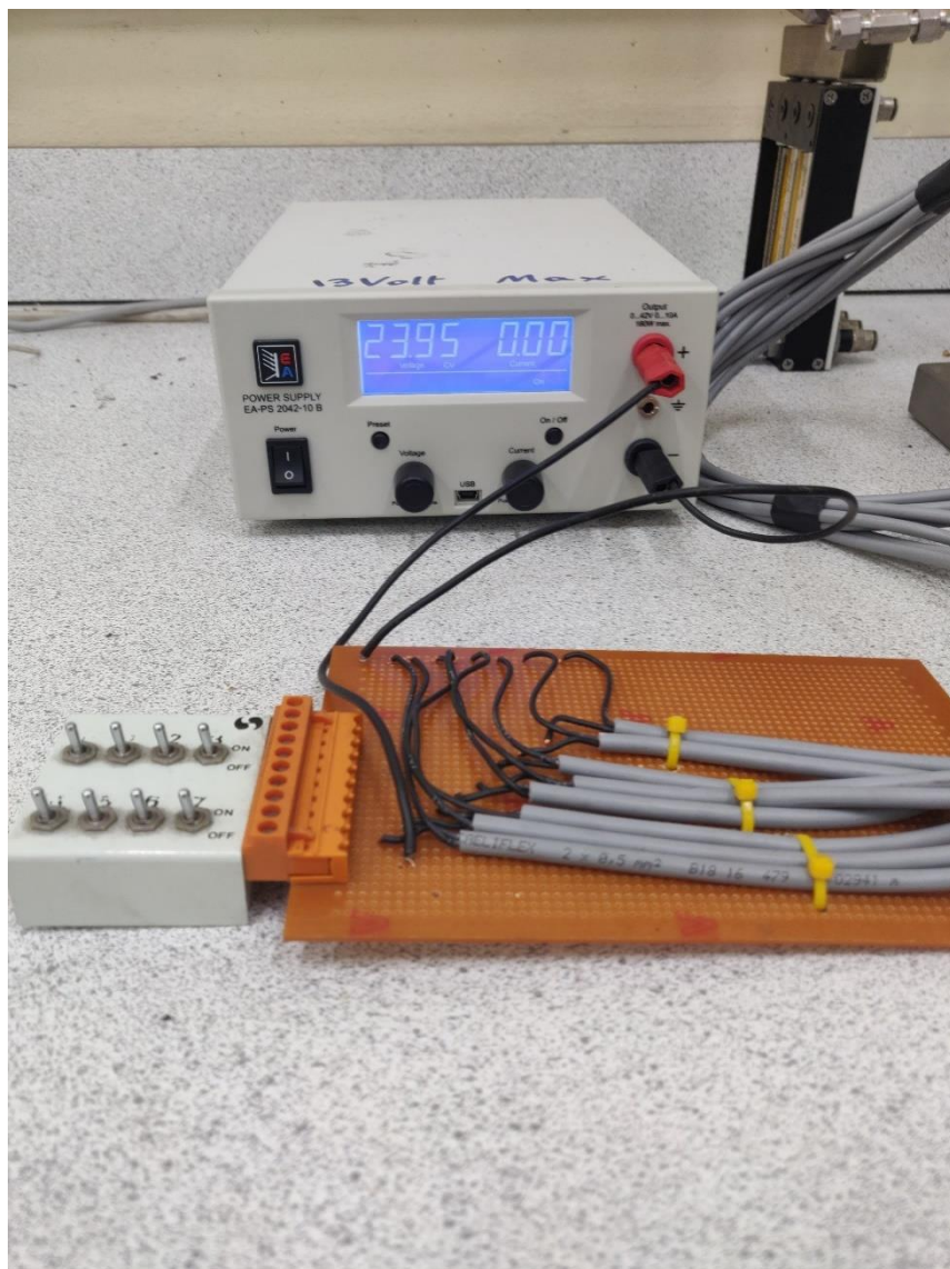
Figure 50 PVSA lab rig electrical switchboard and power supply
