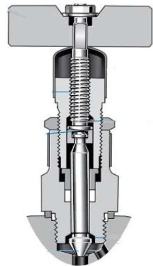
Figure 21 Swagelok Needle Valve
