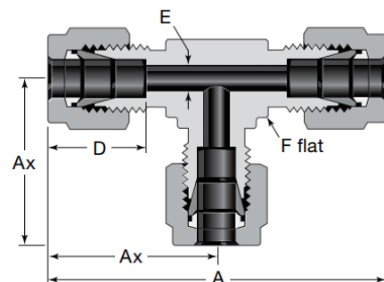
Figure 13 Union T-Fitting
