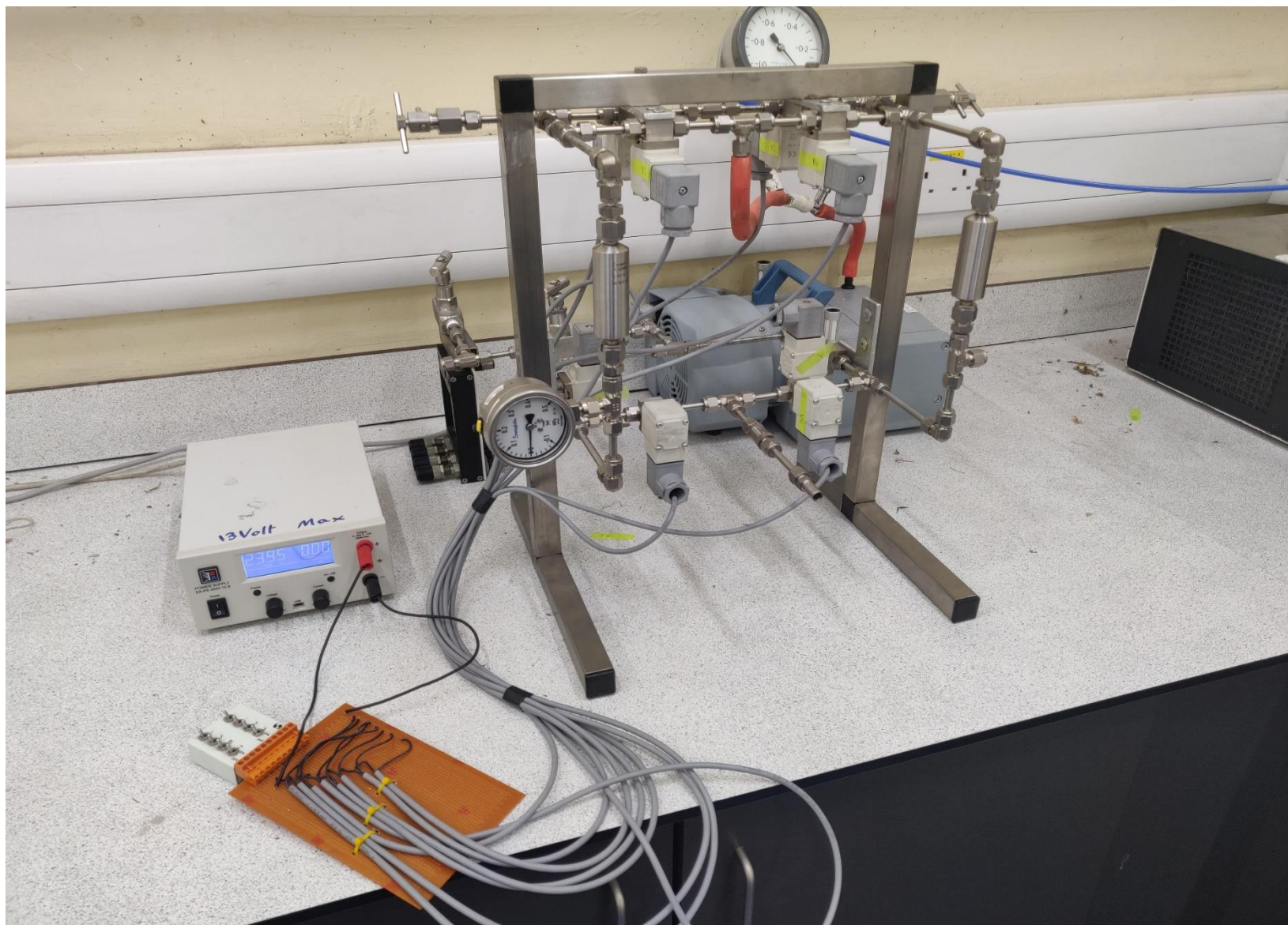
Figure 47 Assembled rig
