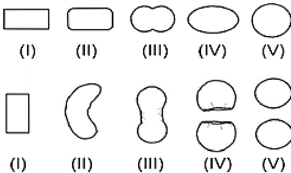
Figure 46 Mechanisms of spheronisation of cylindrical pellets proposed by Rowe (upper) and Baert (lower)
