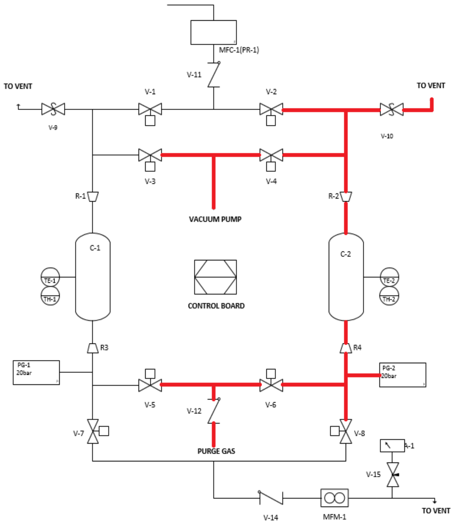
Figure 31 HAZOP Node 2 - Desorption
