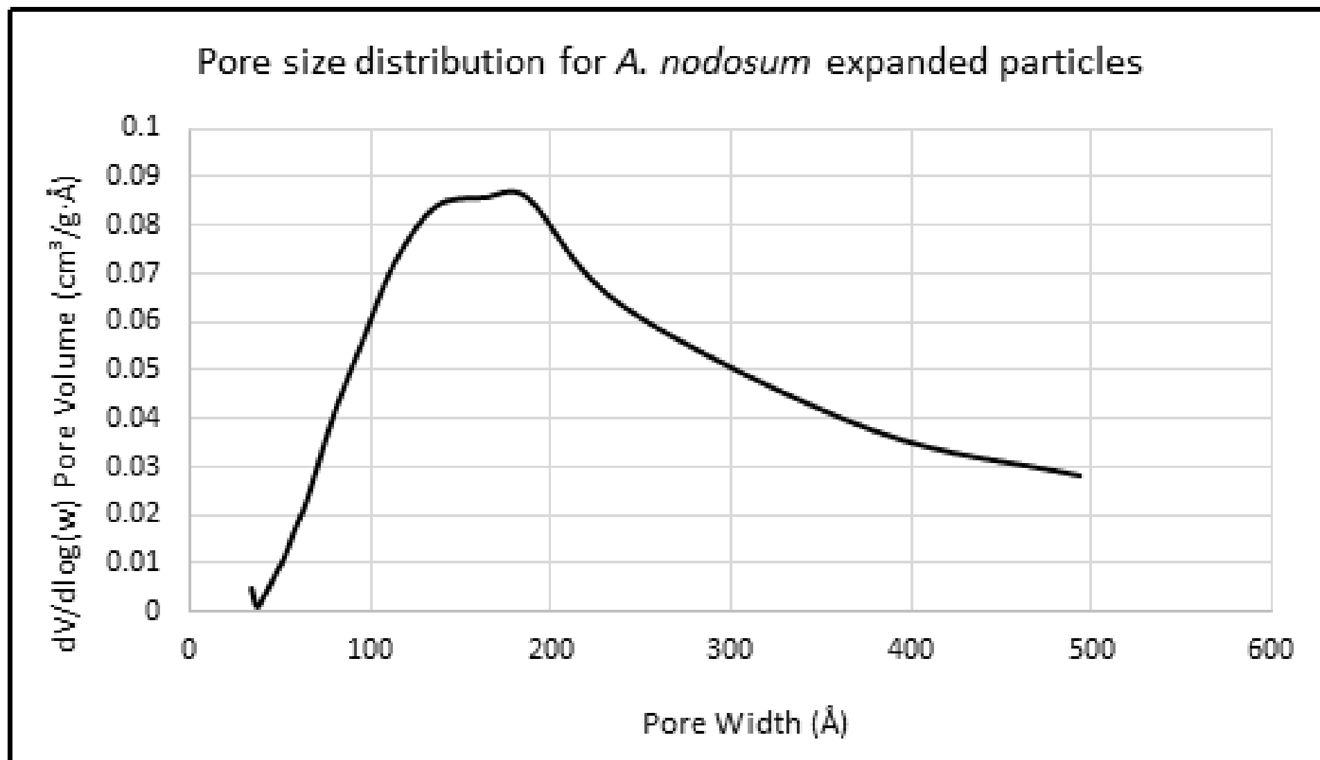
Figure 56 Pore size distribution graph for expanded A. nodosum particles
