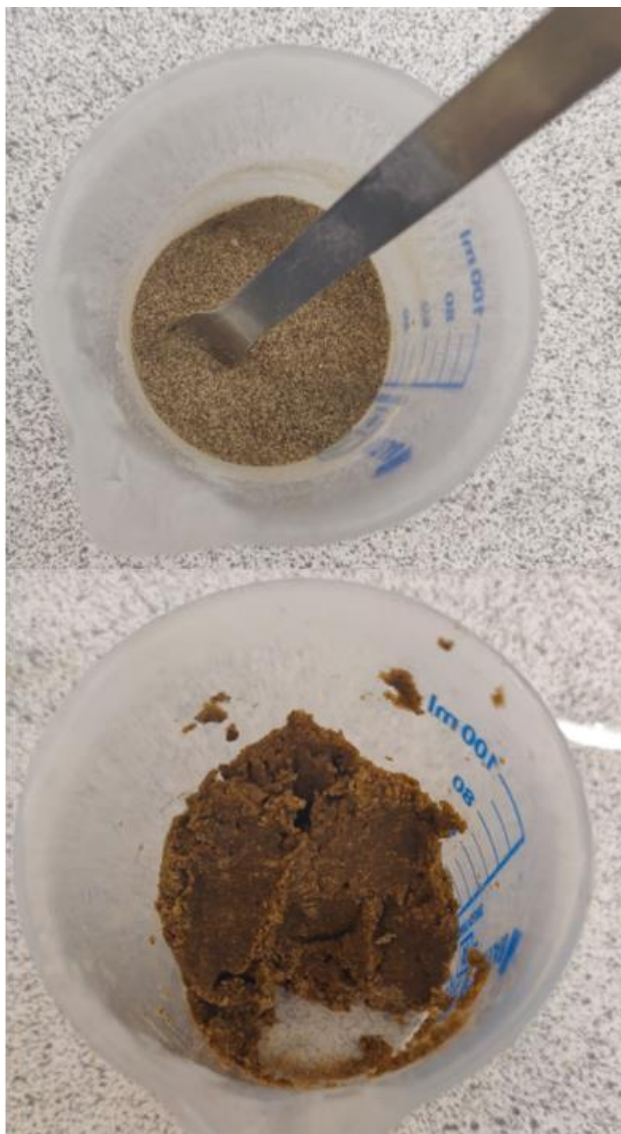
Figure 60 Powder blend (top) and adsorbent paste (bottom)
