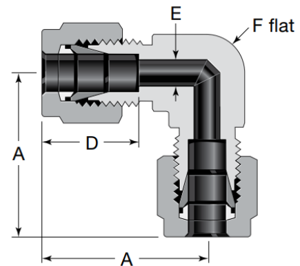
Figure 14 Swagelok 90° Union
