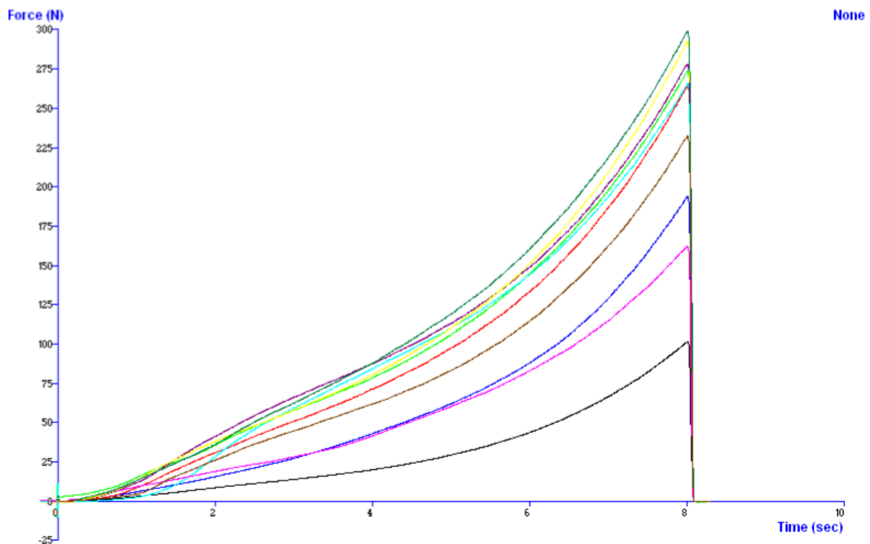
Figure 69 Force v Time graph (compressive strength) for 3mm diameter Hexagonal Prism pellets (10 units, Batch 1)
