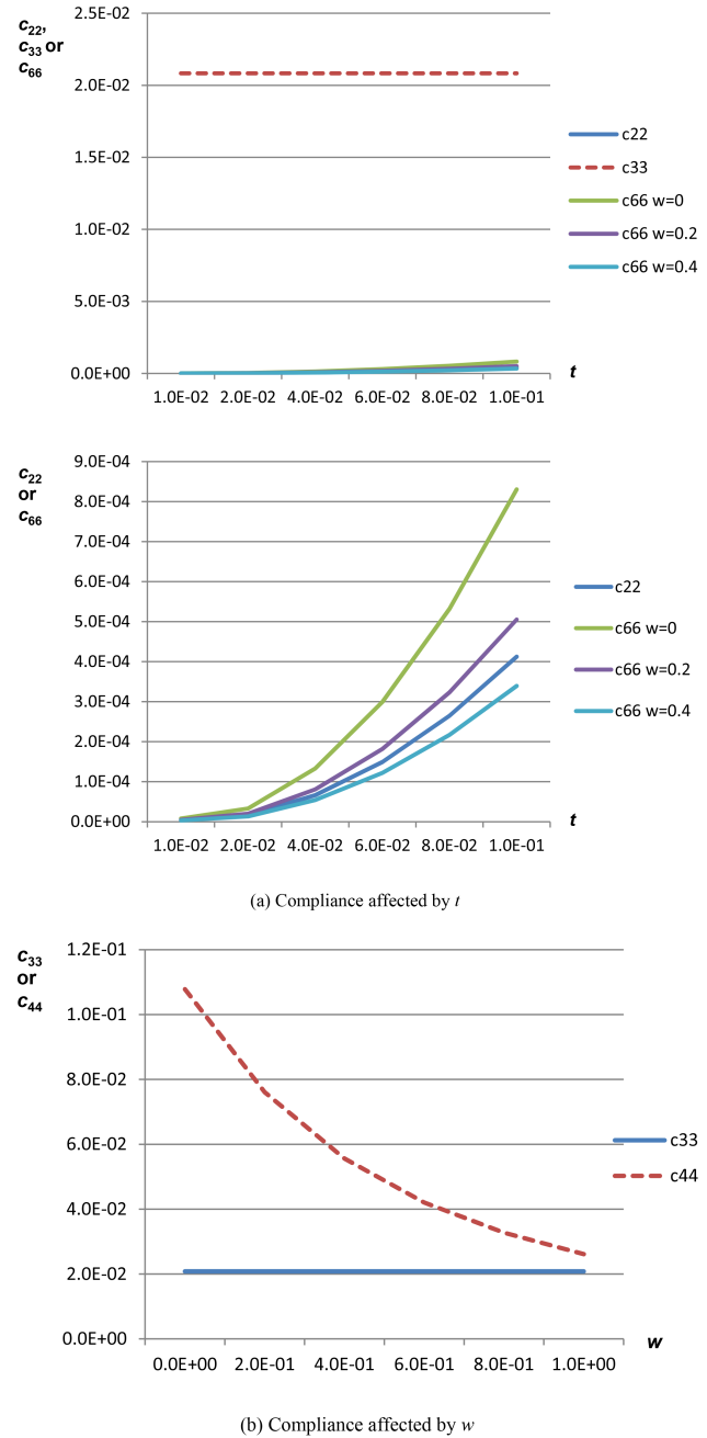
Figure 4. Compliance comparisons of symmetric 4-beam mechanism.
