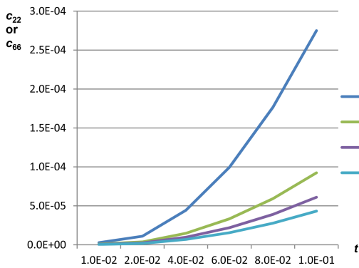
(a) Compliance affected by t
