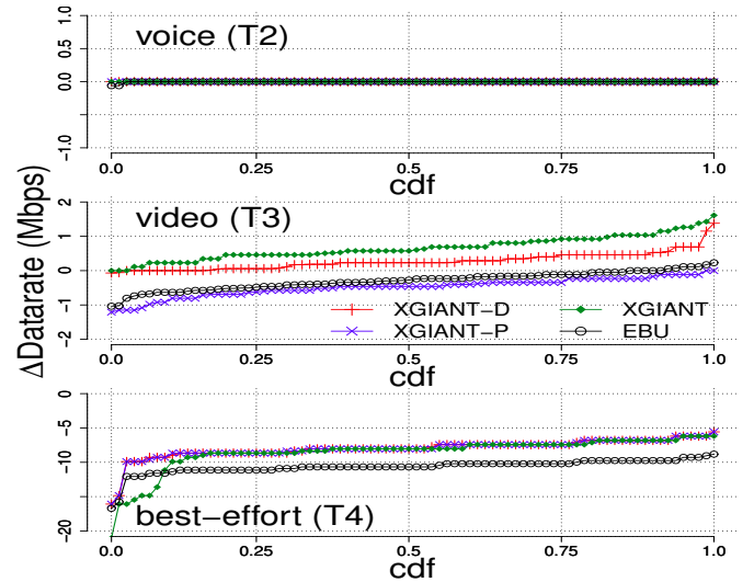
Fig. 12. Difference in mean datarate in 80-eNB scenario
