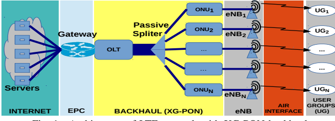
Fig. 1. Architecture of LTE network with XG-PON backhaul
