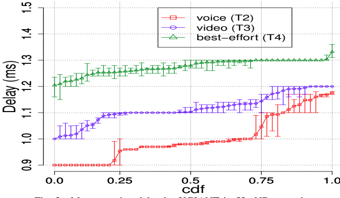
Fig. 3. Mean queuing-delay by XGIANT in 52-eNB scenario
