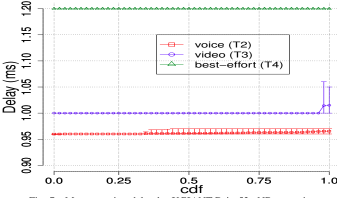
Fig. 7. Mean queuing-delay by XGIANT-D in 52-eNB scenario
