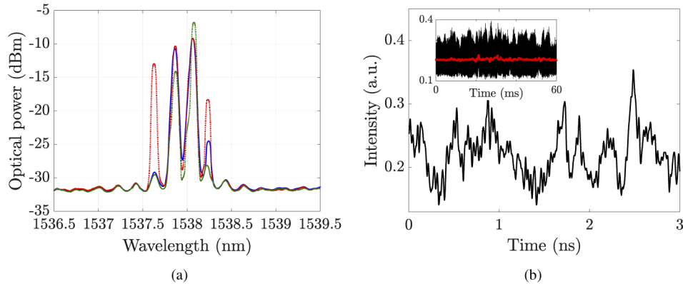
Fig. 4. (a) OSA of 3 captures of lasing spectrum at ~10 second intervals. (b) Laser intensity time trace ns scale showing large power fluctuations. Inset: ms scale intensity (black) and smoothed average intensity (red).
